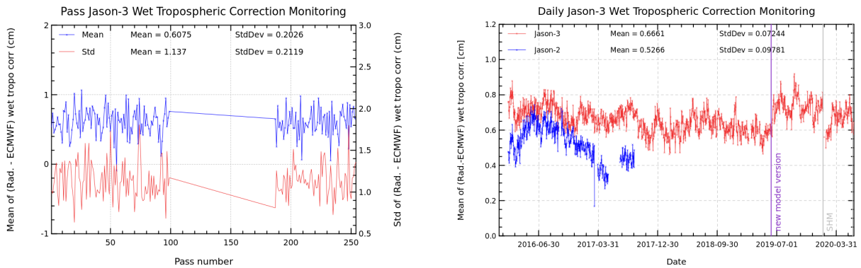
FIGURE 11 – Pass monitoring of wet troposphere differences between radiometer and ECMWF model for Jason-3 cycle 160 (left) and Jason-3 versus Jason-2 daily monitoring of wet troposphere differences between radiometer and ECMWF model (right).
