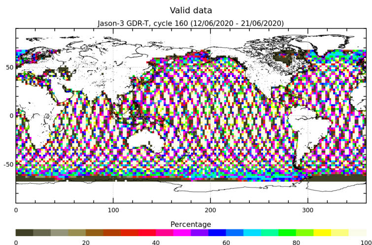
FIGURE 3 – Percentage of valid measurements for cycle 160.
