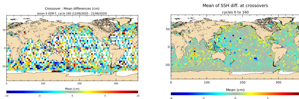
FIGURE 12 – Mean SSH at crossovers for cycle 160 (left) and over the whole Jason-3 period (right).
