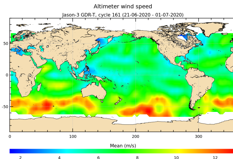
FIGURE 9 – Altimeter wind speed for cycle 161.
