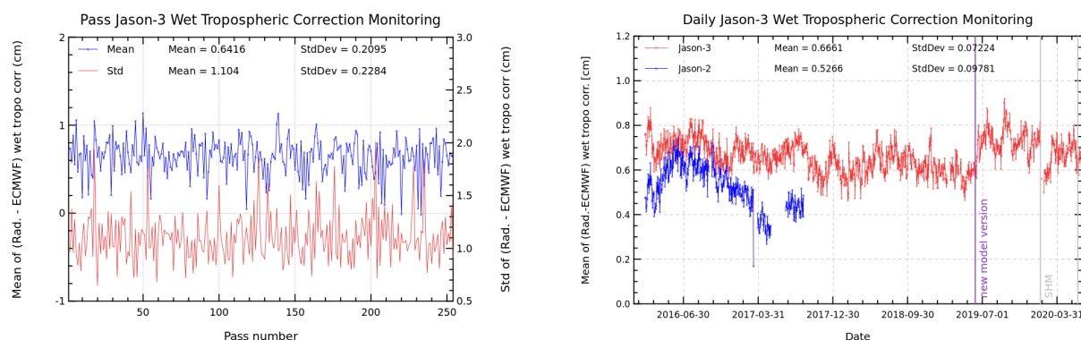
FIGURE 11 – Pass monitoring of wet troposphere differences between radiometer and ECMWF model for Jason-3 cycle 161 (left) and Jason-3 versus Jason-2 daily monitoring of wet troposphere differences between radiometer and ECMWF model (right).
