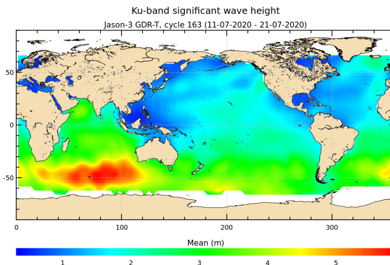
FIGURE 5 – Significant wave height for cycle 163.
