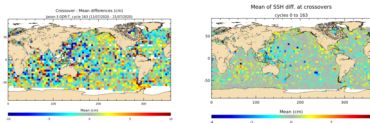
FIGURE 12 – Mean SSH at crossovers for cycle 163 (left) and over the whole Jason-3 period (right).
