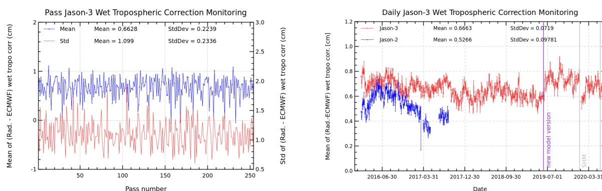
FIGURE 11 – Pass monitoring of wet troposphere differences between radiometer and ECMWF model for Jason-3 cycle 163 (left) and Jason-3 versus Jason-2 daily monitoring of wet troposphere differences between radiometer and ECMWF model (right).
