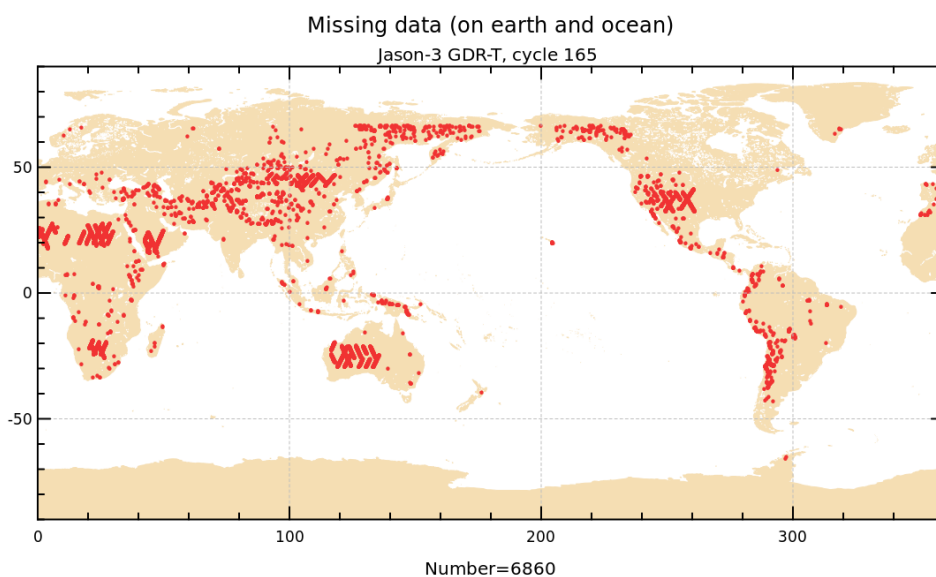
FIGURE 1 – Missing measurements for cycle 165.
