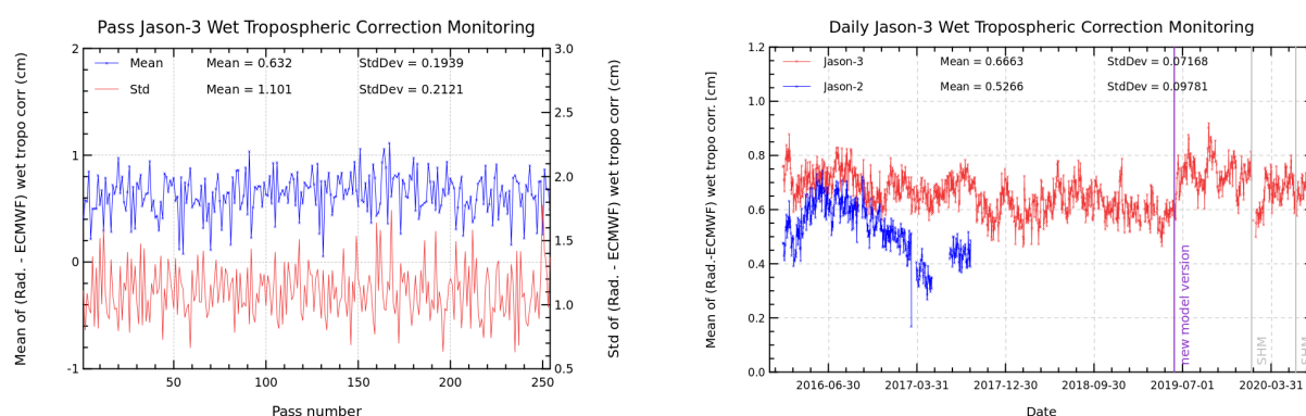
FIGURE 11 – Pass monitoring of wet troposphere differences between radiometer and ECMWF model for Jason-3 cycle 165 (left) and Jason-3 versus Jason-2 daily monitoring of wet troposphere differences between radiometer and ECMWF model (right).
