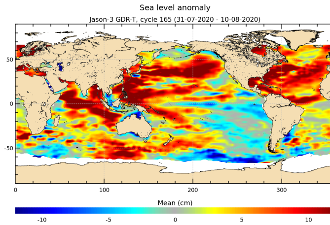
FIGURE 17 – Sea level anomaly relative to MSS for cycle 165.
