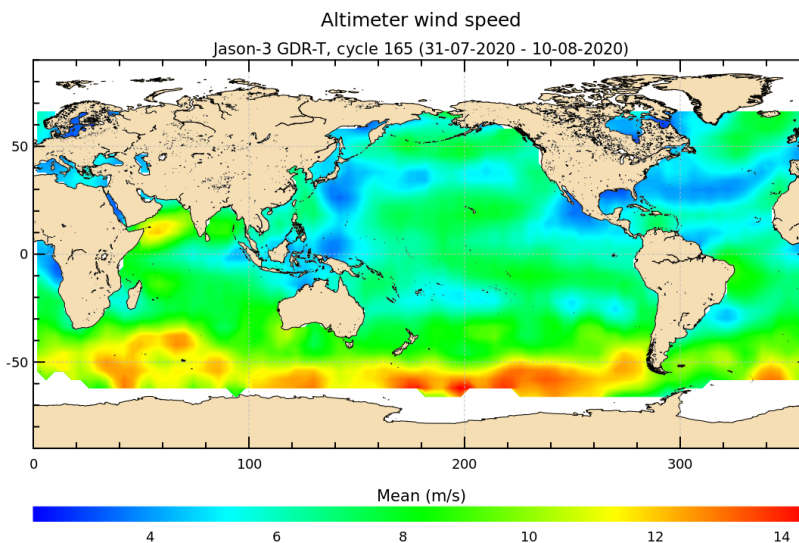
FIGURE 9 – Altimeter wind speed for cycle 165.
