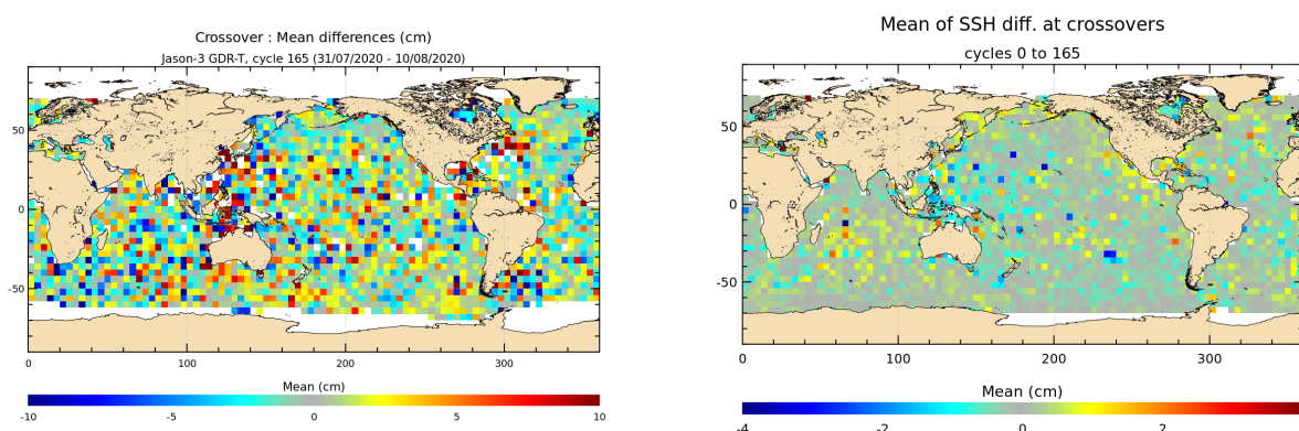
FIGURE 12 – Mean SSH at crossovers for cycle 165 (left) and over the whole Jason-3 period (right).
