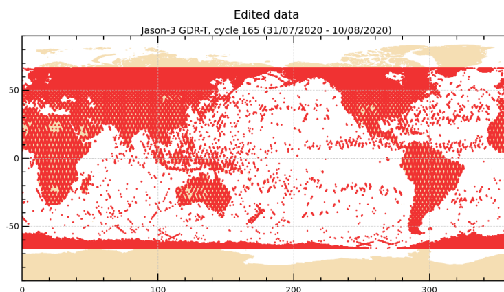
FIGURE 2 – Edited measurements for cycle 165.
