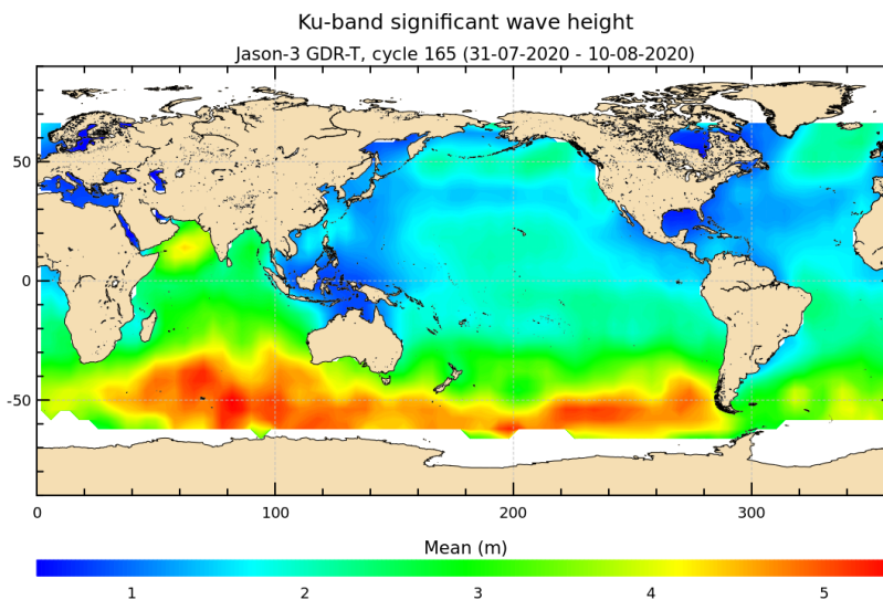
FIGURE 5 – Significant wave height for cycle 165.
