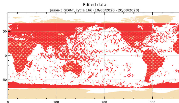
FIGURE 2 – Edited measurements for cycle 166.
