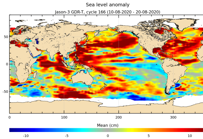
FIGURE 17 – Sea level anomaly relative to MSS for cycle 166.
