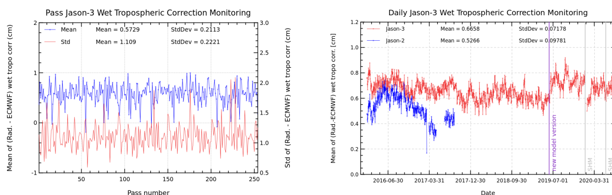
FIGURE 11 – Pass monitoring of wet troposphere differences between radiometer and ECMWF model for Jason-3 cycle 166 (left) and Jason-3 versus Jason-2 daily monitoring of wet troposphere differences between radiometer and ECMWF model (right).
