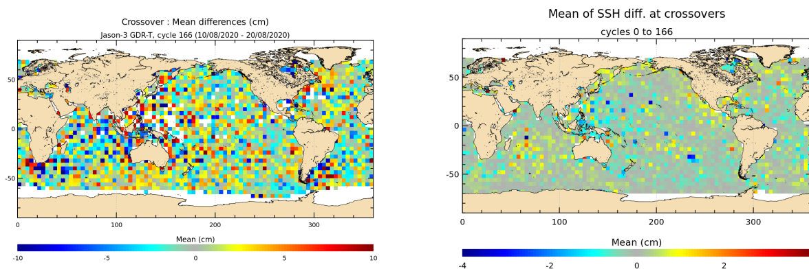
FIGURE 12 – Mean SSH at crossovers for cycle 166 (left) and over the whole Jason-3 period (right).
