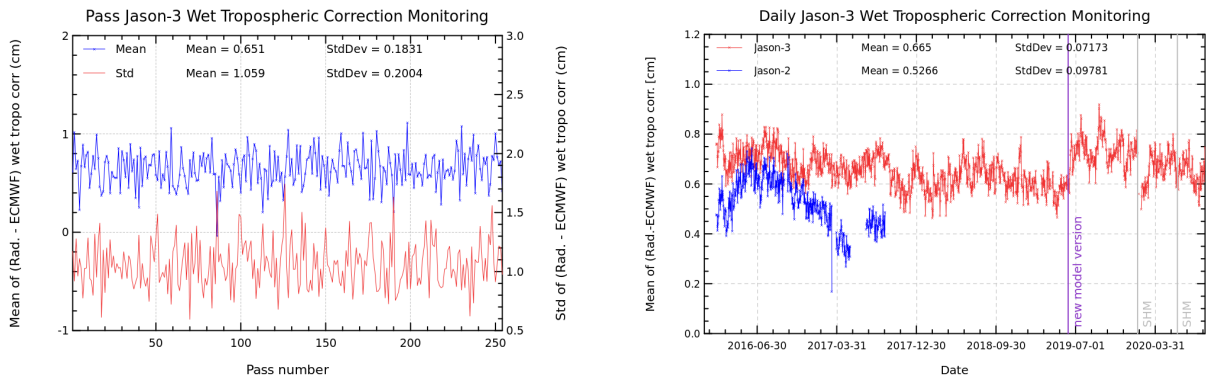
FIGURE 11 – Pass monitoring of wet troposphere differences between radiometer and ECMWF model for Jason-3 cycle 169 (left) and Jason-3 versus Jason-2 daily monitoring of wet troposphere differences between radiometer and ECMWF model (right).
