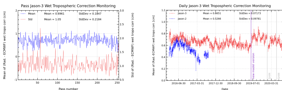
FIGURE 11 – Pass monitoring of wet troposphere differences between radiometer and ECMWF model for Jason-3 cycle 170 (left) and Jason-3 versus Jason-2 daily monitoring of wet troposphere differences between radiometer and ECMWF model (right).
