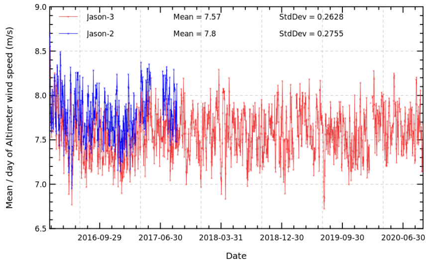
FIGURE 10 – Daily monitoring of altimeter wind speed for Jason-2 and Jason-3.
