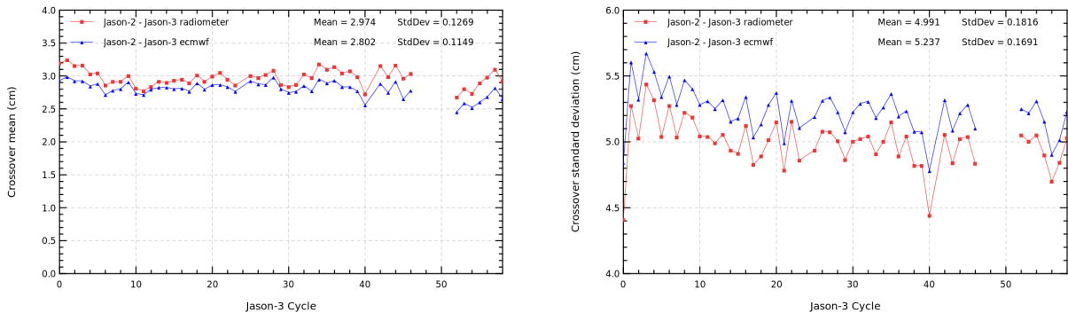
FIGURE 14 – Cyclic monitoring of mean (left) and standard deviation (right) of (Jason-2 – Jason-3) SSH differences at crossovers.
