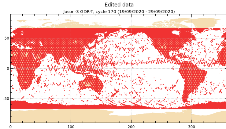
FIGURE 2 – Edited measurements for cycle 170.
