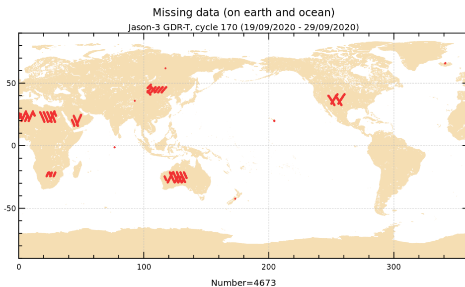
FIGURE 1 – Missing measurements for cycle 170.
