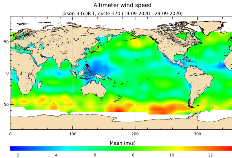
FIGURE 9 – Altimeter wind speed for cycle 170.
