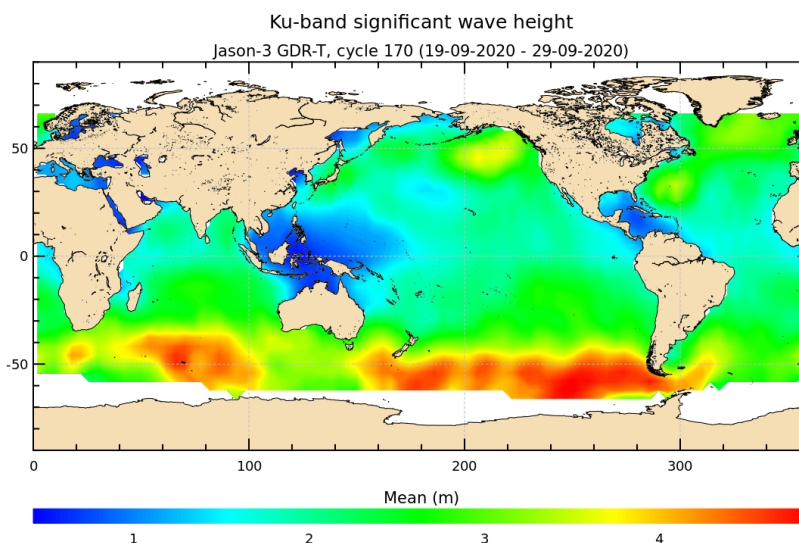
FIGURE 5 – Significant wave height for cycle 170.
