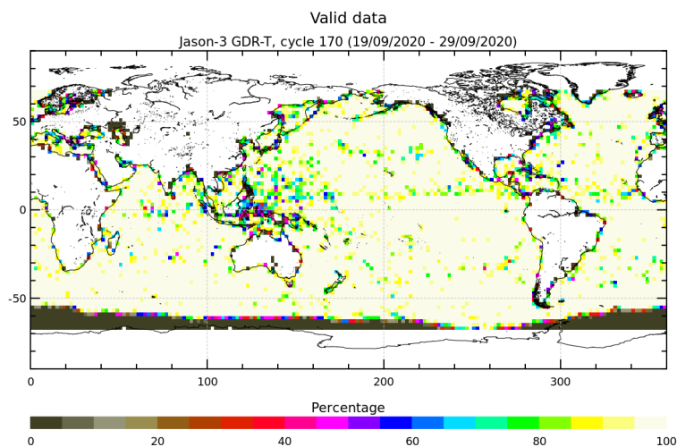
FIGURE 3 – Percentage of valid measurements for cycle 170.
