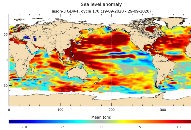
FIGURE 17 – Sea level anomaly relative to MSS for cycle 170.
