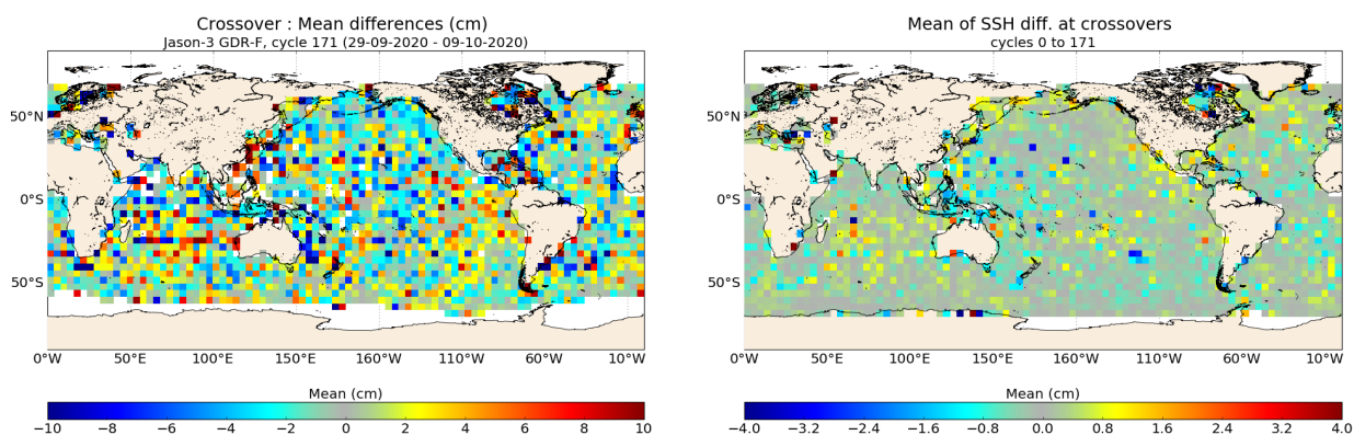
FIGURE 13 – Mean SSH at crossovers for cycle 171 (left) and over the whole Jason-3 period (right).
