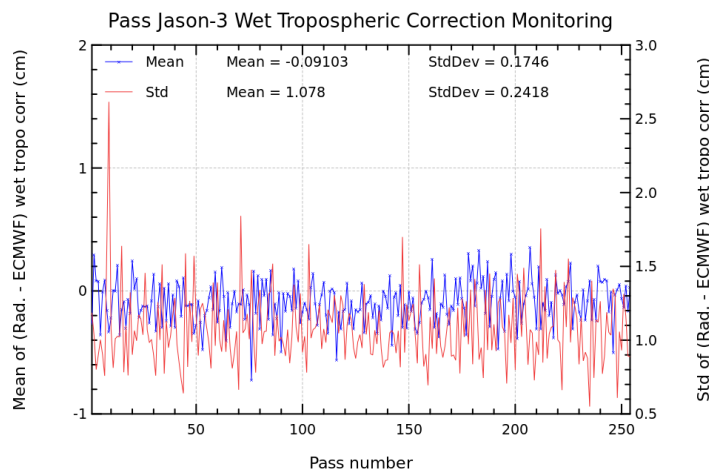
FIGURE 11 – Pass monitoring of wet troposphere differences between radiometer and ECMWF model for Jason-3 cycle 171
