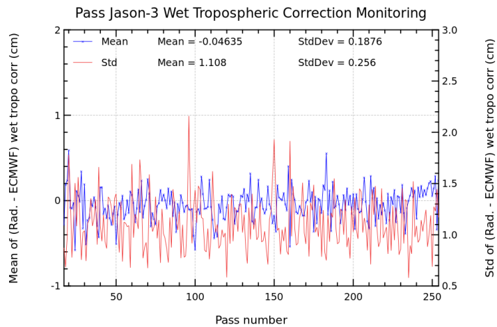
FIGURE 11 – Pass monitoring of wet troposphere differences between radiometer and ECMWF model for Jason-3 cycle 174
