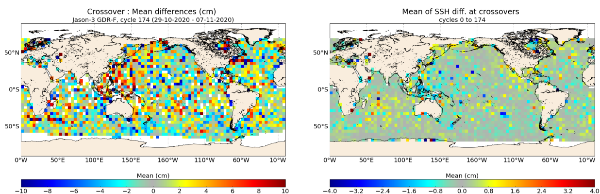
FIGURE 13 – Mean SSH at crossovers for cycle 174 (left) and over the whole Jason-3 period (right).
