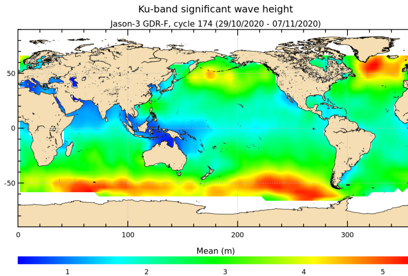
FIGURE 5 – Significant wave height for cycle 174.
