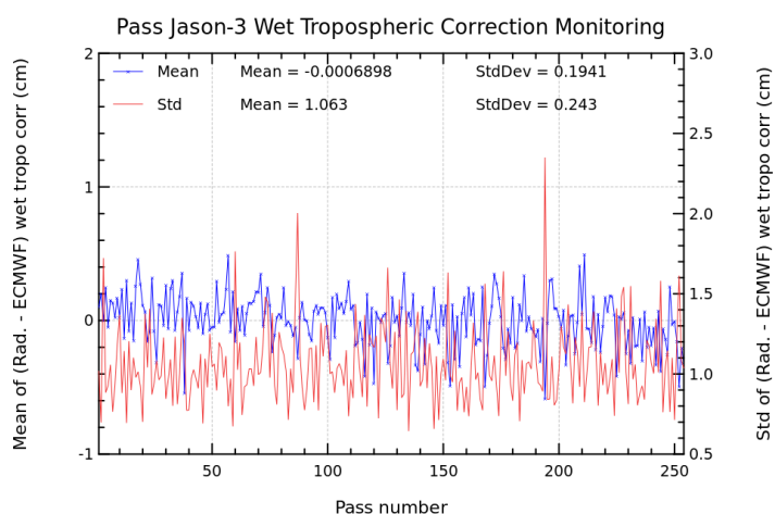
FIGURE 11 – Pass monitoring of wet troposphere differences between radiometer and ECMWF model for Jason-3 cycle 175
