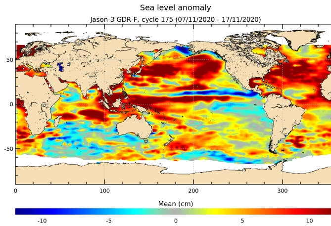
FIGURE 18 – Sea level anomaly relative to MSS for cycle 175.
