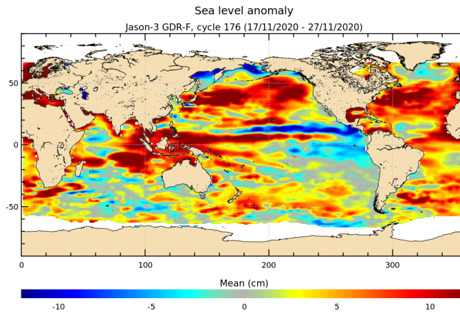
FIGURE 18 – Sea level anomaly relative to MSS for cycle 176.
