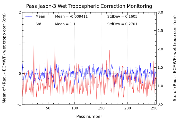
FIGURE 11 – Pass monitoring of wet troposphere differences between radiometer and ECMWF model for Jason-3 cycle 176
