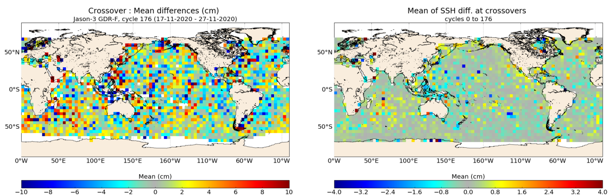
FIGURE 13 – Mean SSH at crossovers for cycle 176 (left) and over the whole Jason-3 period (right).
