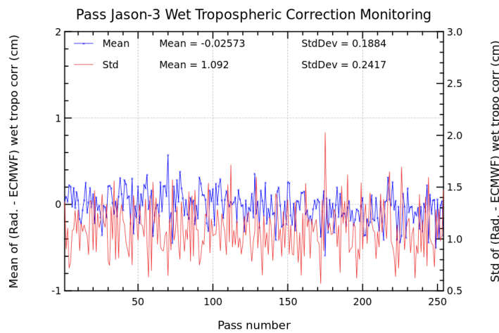
FIGURE 11 – Pass monitoring of wet troposphere differences between radiometer and ECMWF model for Jason-3 cycle 177
