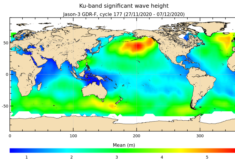
FIGURE 5 – Significant wave height for cycle 177.
