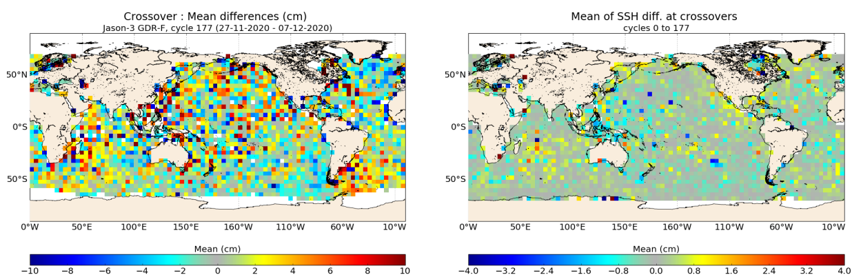
FIGURE 13 – Mean SSH at crossovers for cycle 177 (left) and over the whole Jason-3 period (right).
