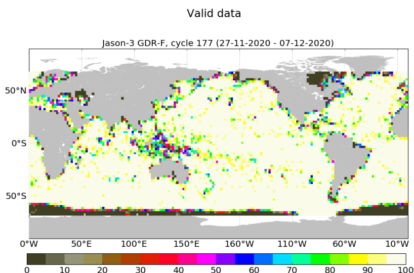
FIGURE 3 – Percentage of valid measurements for cycle 177.
