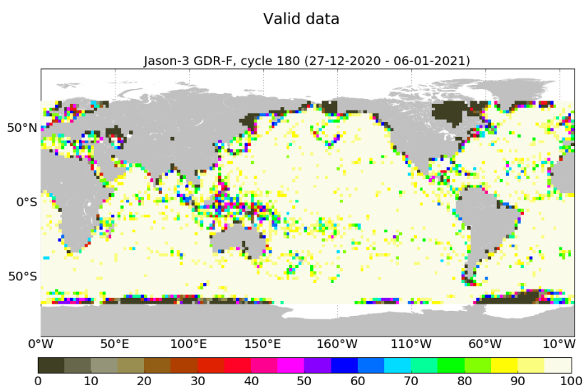
FIGURE 3 – Percentage of valid measurements for cycle 180.
