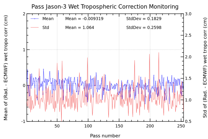
FIGURE 11 – Pass monitoring of wet troposphere differences between radiometer and ECMWF model for Jason-3 cycle 180
