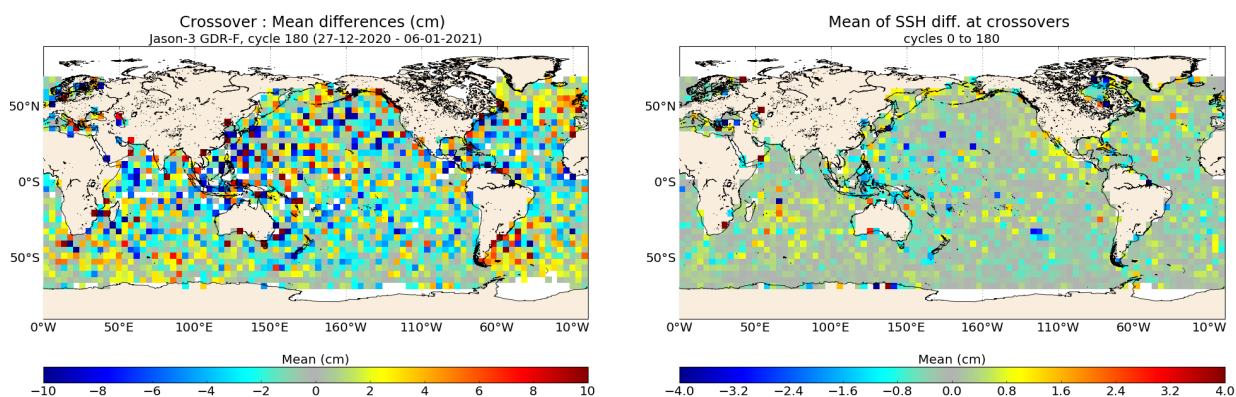
FIGURE 13 – Mean SSH at crossovers for cycle 180 (left) and over the whole Jason-3 period (right).
