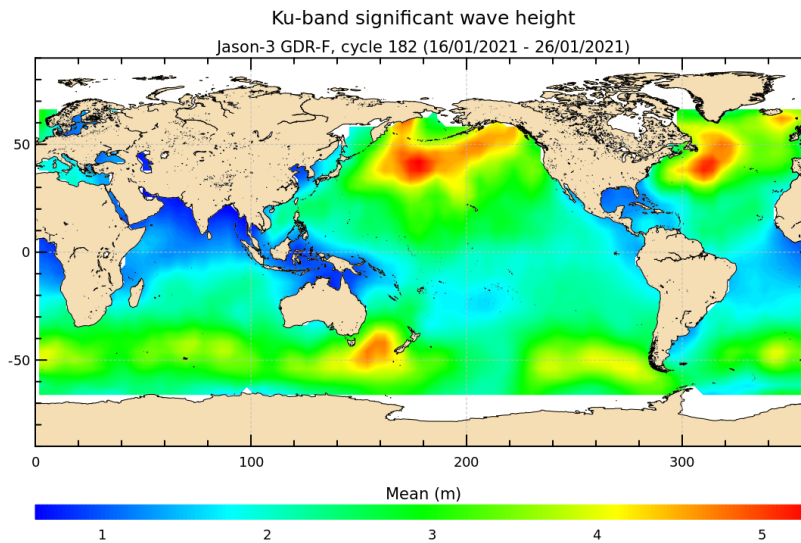
FIGURE 5 – Significant wave height for cycle 182.
