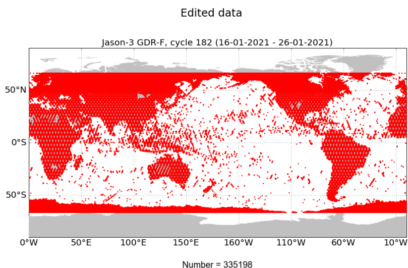
FIGURE 2 – Edited measurements for cycle 182.
