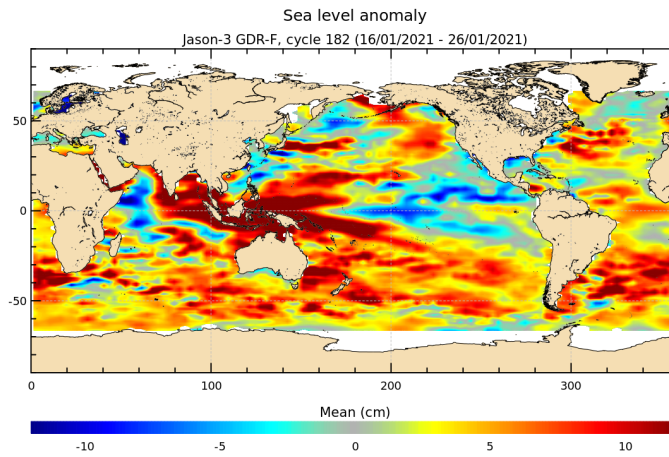
FIGURE 18 – Sea level anomaly relative to MSS for cycle 182.
