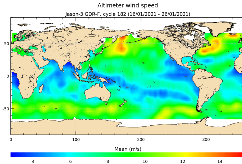
FIGURE 9 – Altimeter wind speed for cycle 182.
