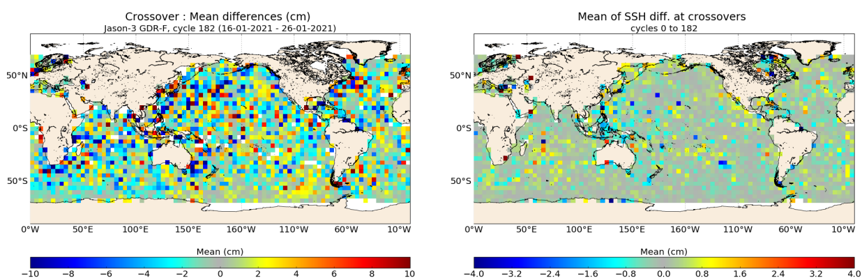
FIGURE 13 – Mean SSH at crossovers for cycle 182 (left) and over the whole Jason-3 period (right).
