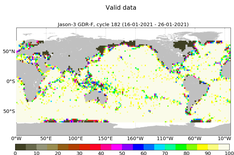
FIGURE 3 – Percentage of valid measurements for cycle 182.
