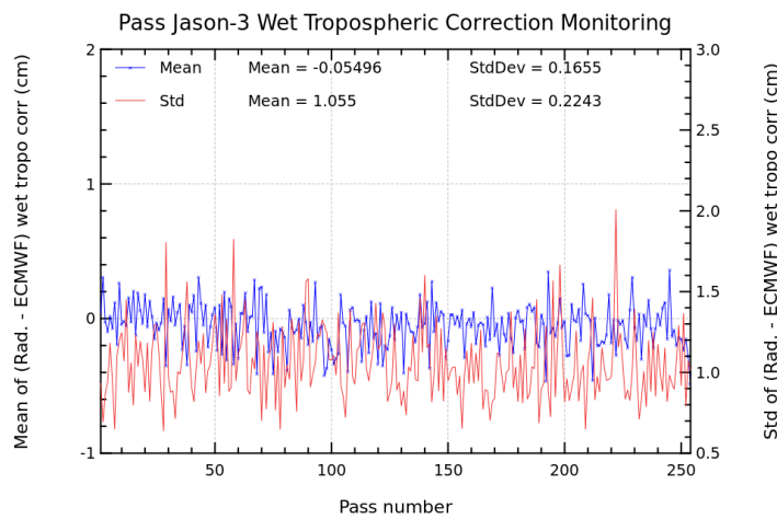
FIGURE 11 – Pass monitoring of wet troposphere differences between radiometer and ECMWF model for Jason-3 cycle 182
