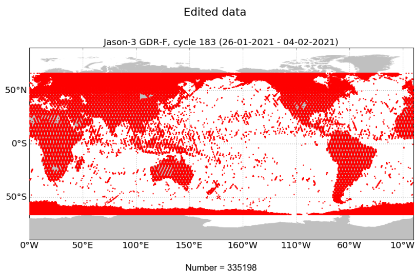
FIGURE 2 – Edited measurements for cycle 183.
