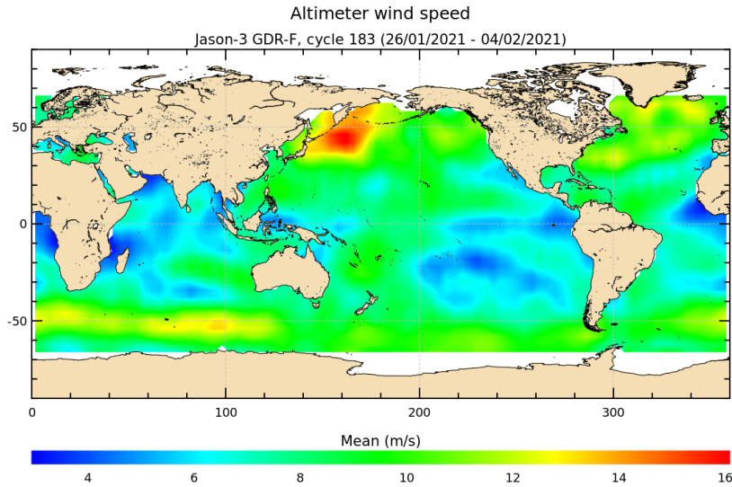
FIGURE 9 – Altimeter wind speed for cycle 183.
