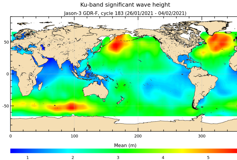
FIGURE 5 – Significant wave height for cycle 183.
