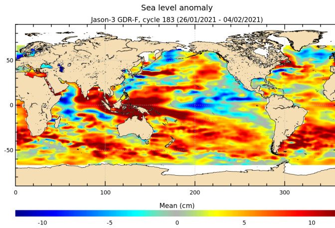
FIGURE 18 – Sea level anomaly relative to MSS for cycle 183.
