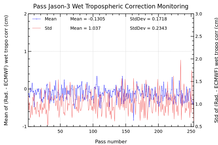
FIGURE 11 – Pass monitoring of wet troposphere differences between radiometer and ECMWF model for Jason-3 cycle 183
