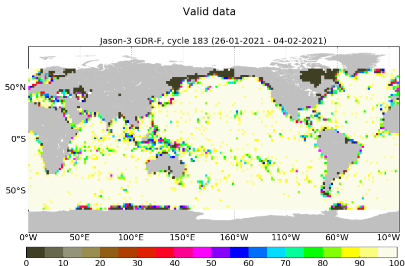
FIGURE 3 – Percentage of valid measurements for cycle 183.
