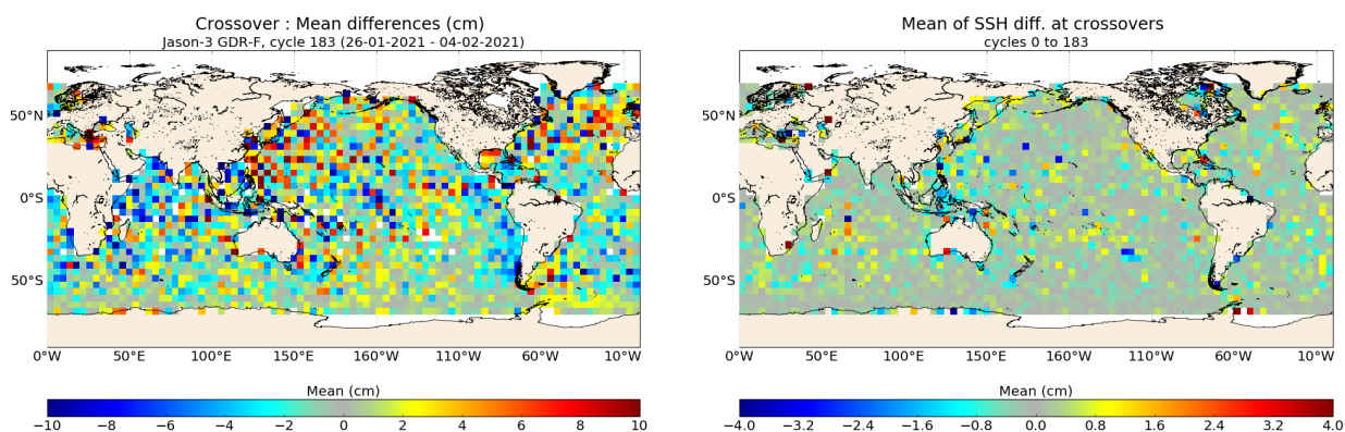
FIGURE 13 – Mean SSH at crossovers for cycle 183 (left) and over the whole Jason-3 period (right).
