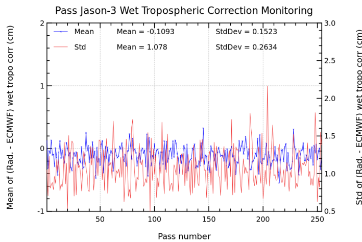
FIGURE 11 – Pass monitoring of wet troposphere differences between radiometer and ECMWF model for Jason-3 cycle 184
