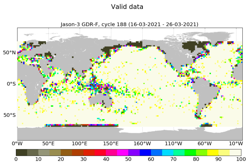
FIGURE 3 – Percentage of valid measurements for cycle 188.
