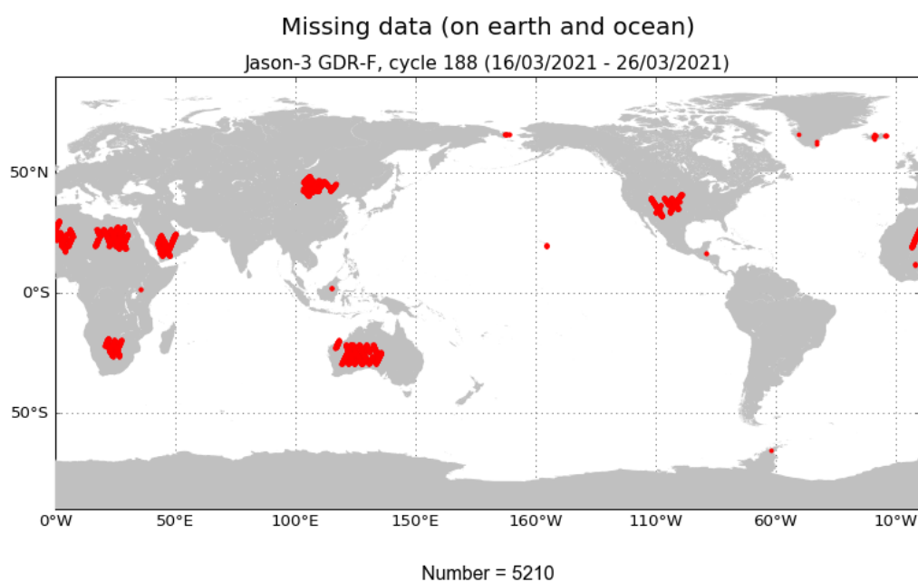
FIGURE 1 – Missing measurements for cycle 188.
