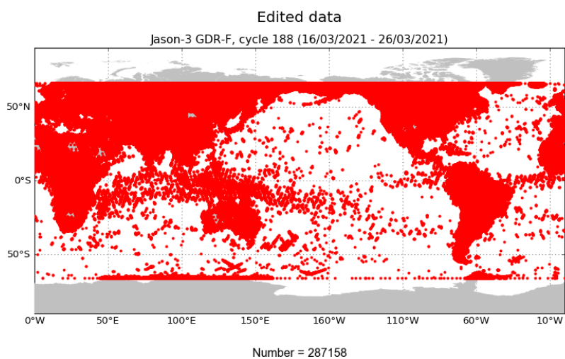
FIGURE 2 – Edited measurements for cycle 188.
