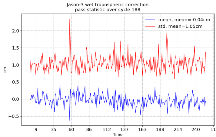
FIGURE 11 – Pass monitoring of wet troposphere differences between radiometer and ECMWF model for Jason-3 cycle 188
