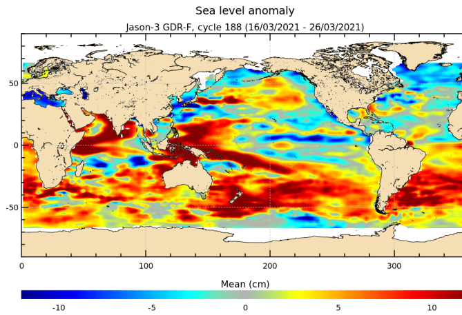
FIGURE 18 – Sea level anomaly relative to MSS for cycle 188.
