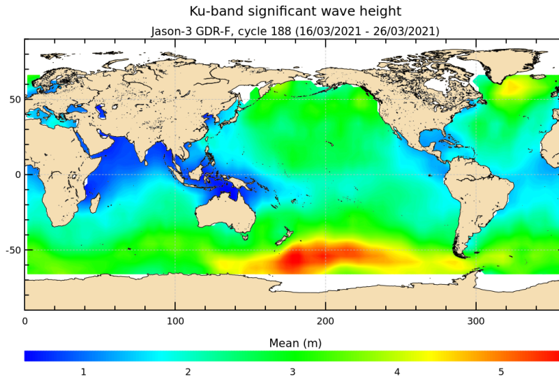
FIGURE 5 – Significant wave height for cycle 188.
