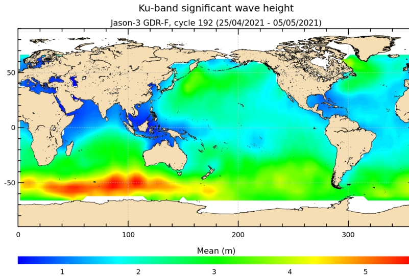
FIGURE 5 – Significant wave height for cycle 192.
