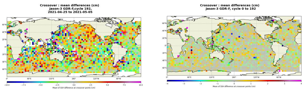
FIGURE 13 – Mean SSH at crossovers for cycle 192 (left) and over the whole Jason-3 period (right).
