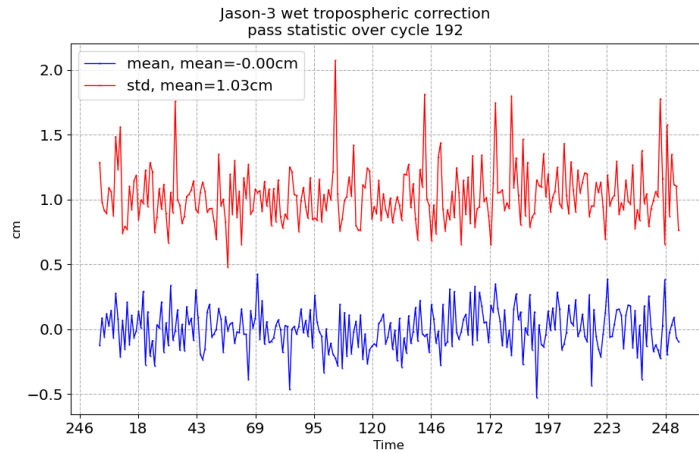
FIGURE 11 – Pass monitoring of wet troposphere differences between radiometer and ECMWF model for Jason-3 cycle 192
