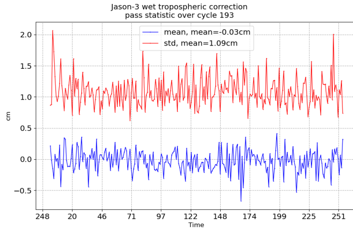
FIGURE 11 – Pass monitoring of wet troposphere differences between radiometer and ECMWF model for Jason-3 cycle 193
