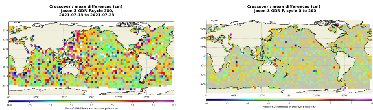
FIGURE 13 – Mean SSH at crossovers for cycle 200 (left) and over the whole Jason-3 period (right).
