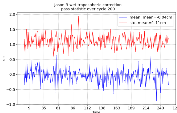
FIGURE 11 – Pass monitoring of wet troposphere differences between radiometer and ECMWF model for Jason-3 cycle 200
