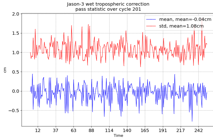
FIGURE 11 – Pass monitoring of wet troposphere differences between radiometer and ECMWF model for Jason-3 cycle 201
