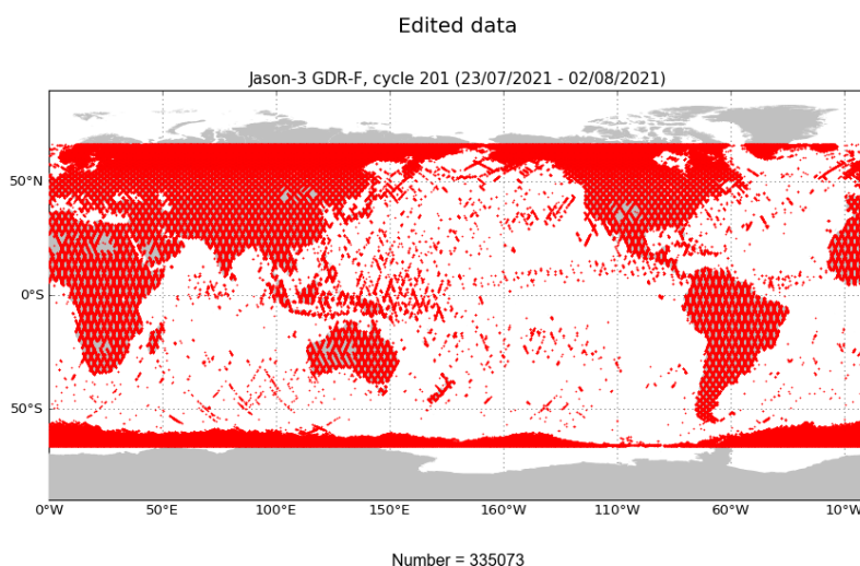
FIGURE 2 – Edited measurements for cycle 201.
