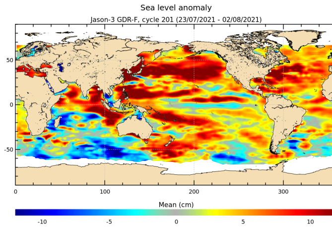
FIGURE 18 – Sea level anomaly relative to MSS for cycle 201.
