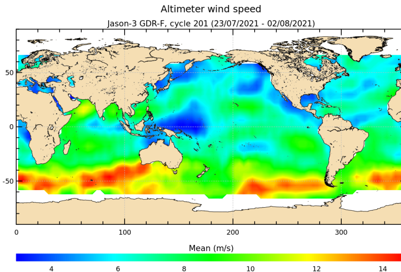
FIGURE 9 – Altimeter wind speed for cycle 201.
