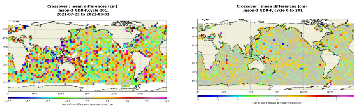
FIGURE 13 – Mean SSH at crossovers for cycle 201 (left) and over the whole Jason-3 period (right).
