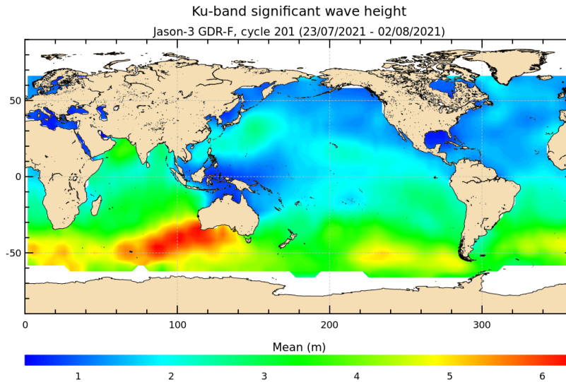
FIGURE 5 – Significant wave height for cycle 201.
