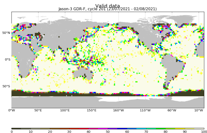
FIGURE 3 – Percentage of valid measurements for cycle 201.
