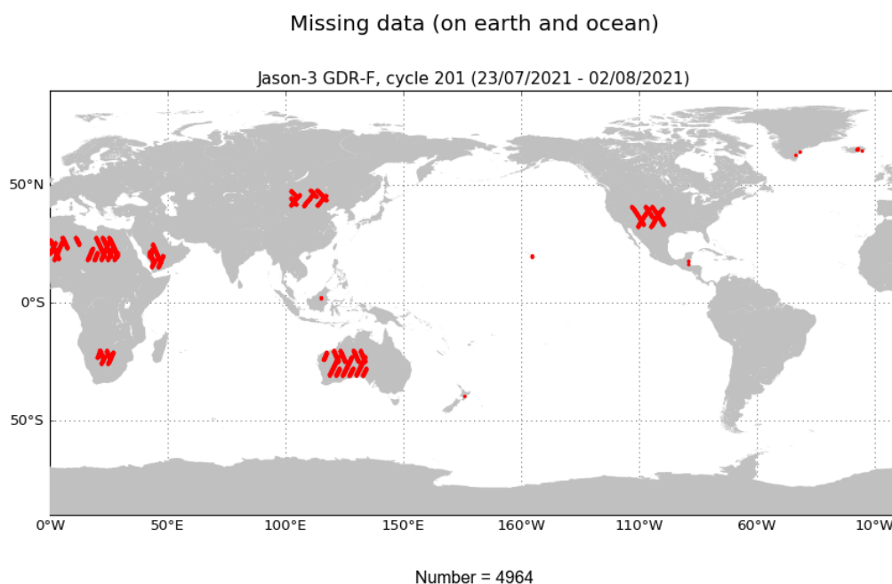
FIGURE 1 – Missing measurements for cycle 201.
