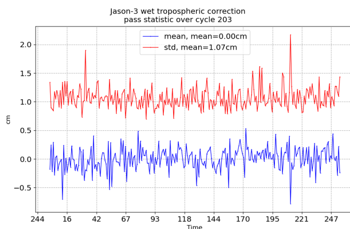
FIGURE 11 – Pass monitoring of wet troposphere differences between radiometer and ECMWF model for Jason-3 cycle 203
