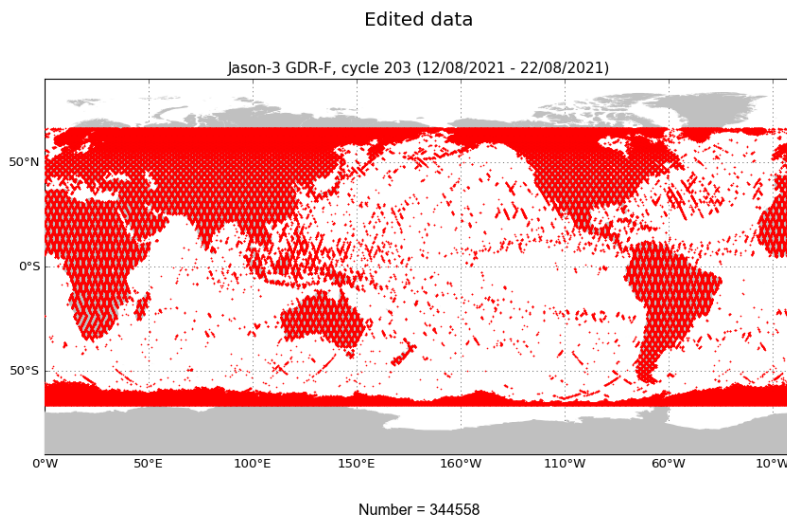
FIGURE 2 – Edited measurements for cycle 203.
