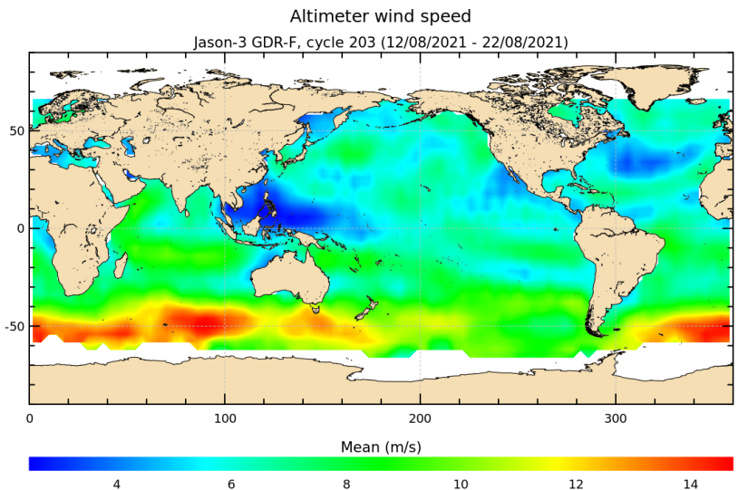
FIGURE 9 – Altimeter wind speed for cycle 203.
