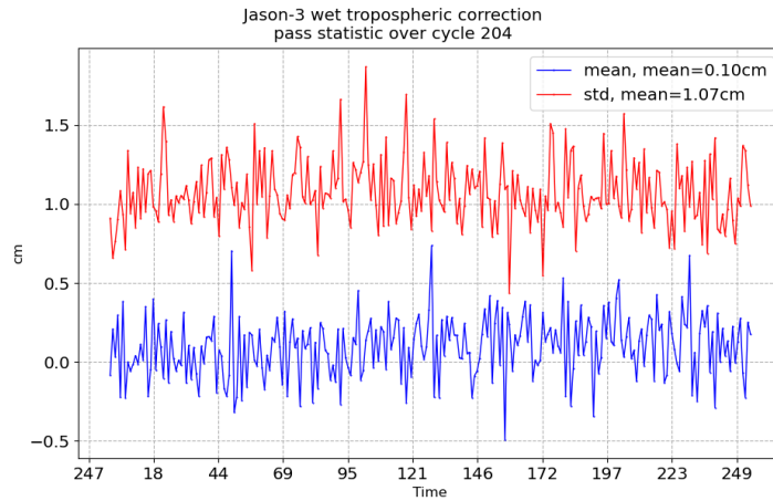
FIGURE 11 – Pass monitoring of wet troposphere differences between radiometer and ECMWF model for Jason-3 cycle 204
