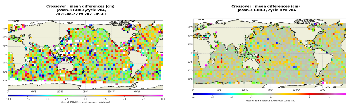
FIGURE 13 – Mean SSH at crossovers for cycle 204 (left) and over the whole Jason-3 period (right).
