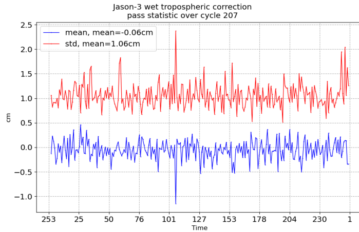
FIGURE 11 – Pass monitoring of wet troposphere differences between radiometer and ECMWF model for Jason-3 cycle 207
