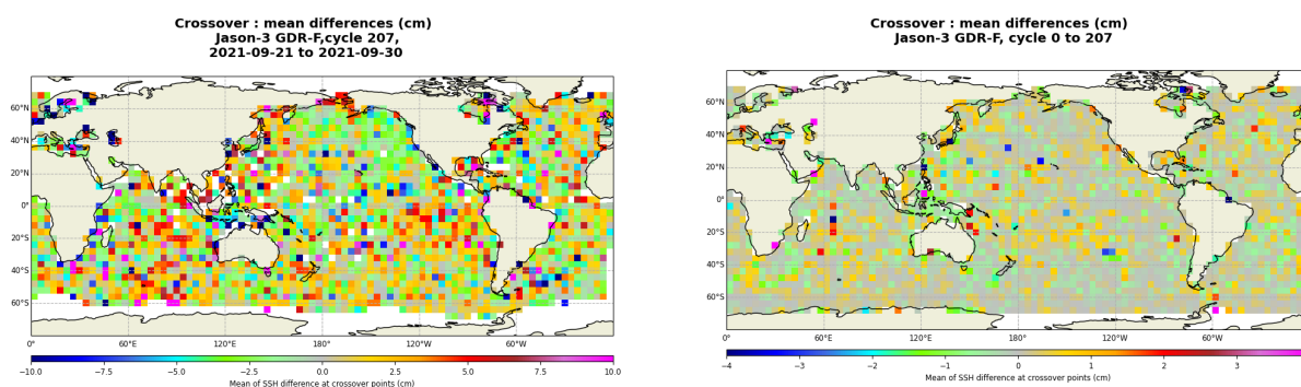
FIGURE 13 – Mean SSH at crossovers for cycle 207 (left) and over the whole Jason-3 period (right).
