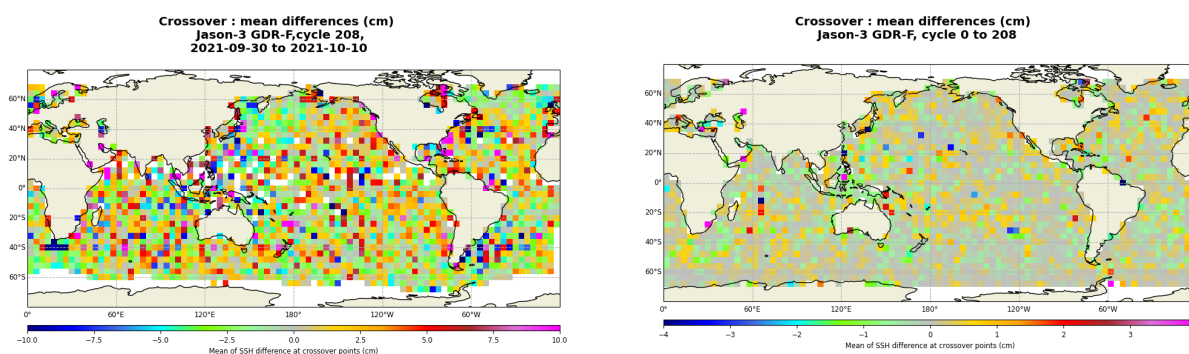
FIGURE 13 – Mean SSH at crossovers for cycle 208 (left) and over the whole Jason-3 period (right).
