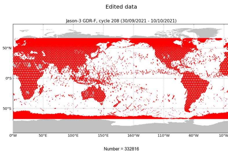
FIGURE 2 – Edited measurements for cycle 208.
