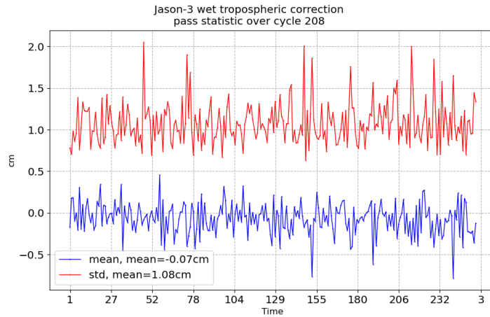
FIGURE 11 – Pass monitoring of wet troposphere differences between radiometer and ECMWF model for Jason-3 cycle 208
