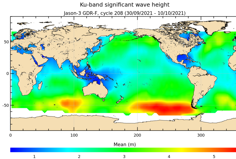
FIGURE 5 – Significant wave height for cycle 208.
