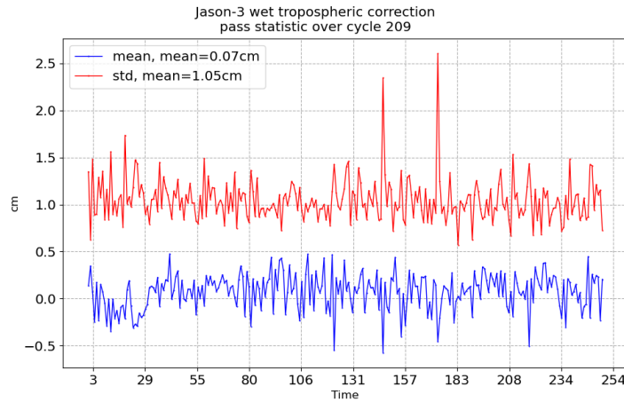
FIGURE 11 – Pass monitoring of wet troposphere differences between radiometer and ECMWF model for Jason-3 cycle 209
