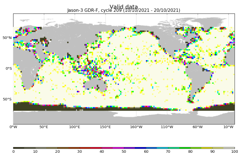
FIGURE 3 – Percentage of valid measurements for cycle 209.
