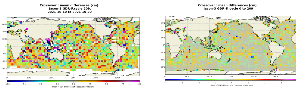
FIGURE 13 – Mean SSH at crossovers for cycle 209 (left) and over the whole Jason-3 period (right).
