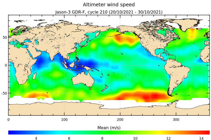
FIGURE 9 – Altimeter wind speed for cycle 210.
