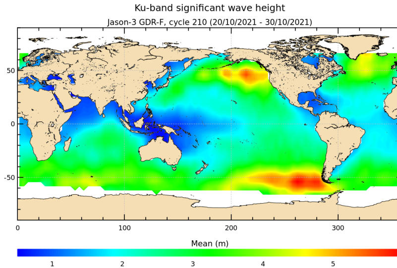
FIGURE 5 – Significant wave height for cycle 210.
