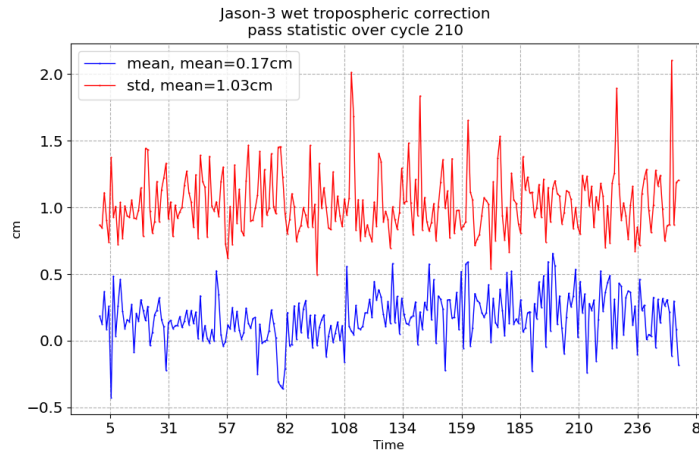
FIGURE 11 – Pass monitoring of wet troposphere differences between radiometer and ECMWF model for Jason-3 cycle 210
