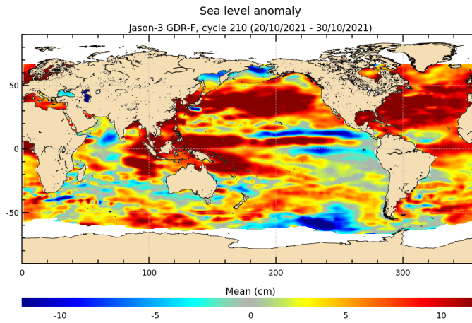
FIGURE 18 – Sea level anomaly relative to MSS for cycle 210.
