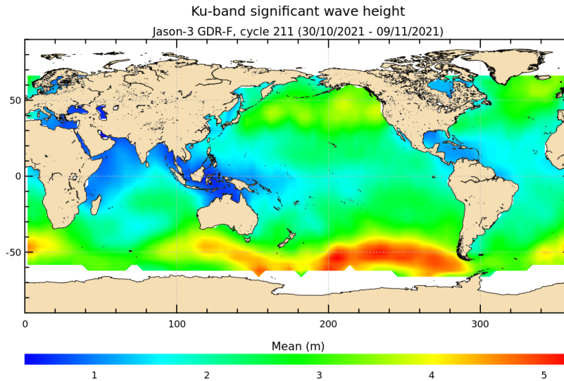
FIGURE 5 – Significant wave height for cycle 211.
