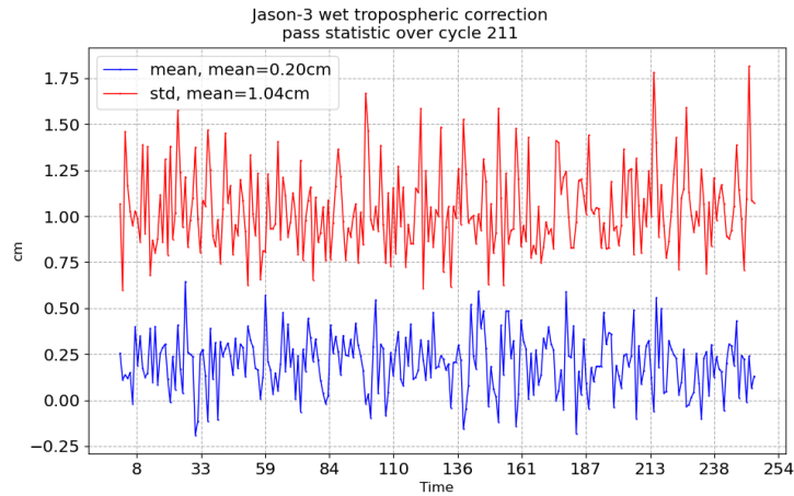
FIGURE 11 – Pass monitoring of wet troposphere differences between radiometer and ECMWF model for Jason-3 cycle 211
