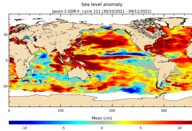
FIGURE 18 – Sea level anomaly relative to MSS for cycle 211.
