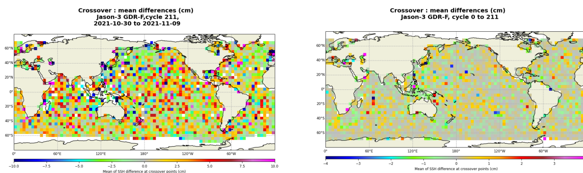
FIGURE 13 – Mean SSH at crossovers for cycle 211 (left) and over the whole Jason-3 period (right).
