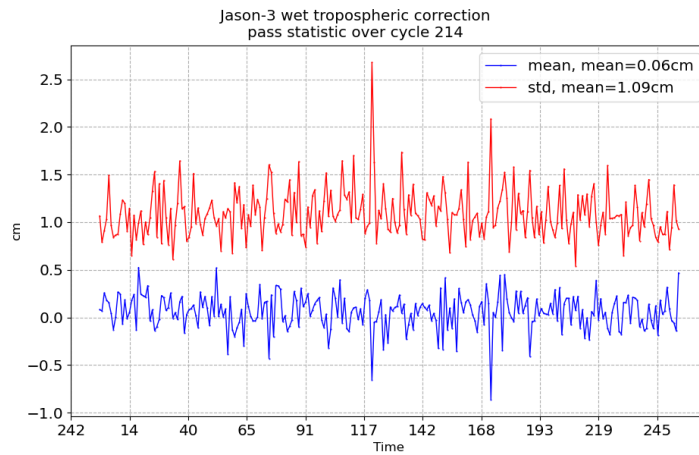
FIGURE 11 – Pass monitoring of wet troposphere differences between radiometer and ECMWF model for Jason-3 cycle 214
