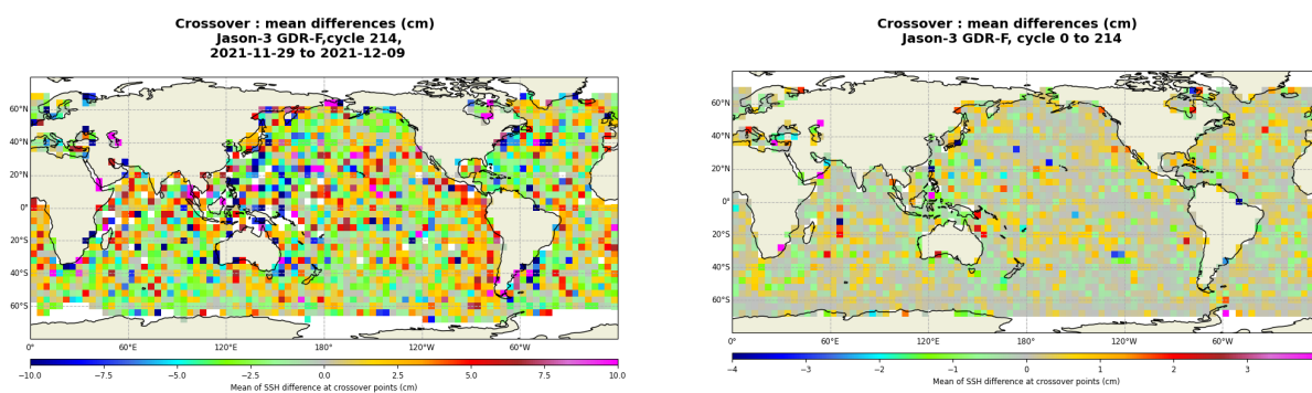
FIGURE 13 – Mean SSH at crossovers for cycle 214 (left) and over the whole Jason-3 period (right).
