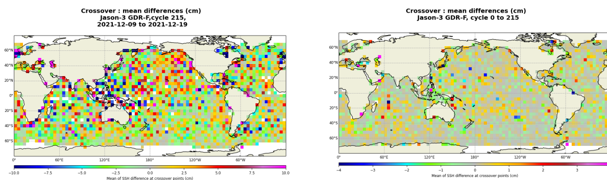
FIGURE 13 – Mean SSH at crossovers for cycle 215 (left) and over the whole Jason-3 period (right).
