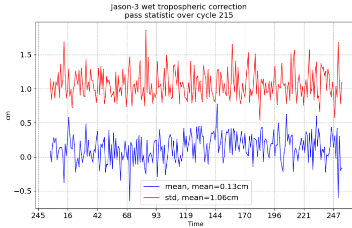
FIGURE 11 – Pass monitoring of wet troposphere differences between radiometer and ECMWF model for Jason-3 cycle 215
