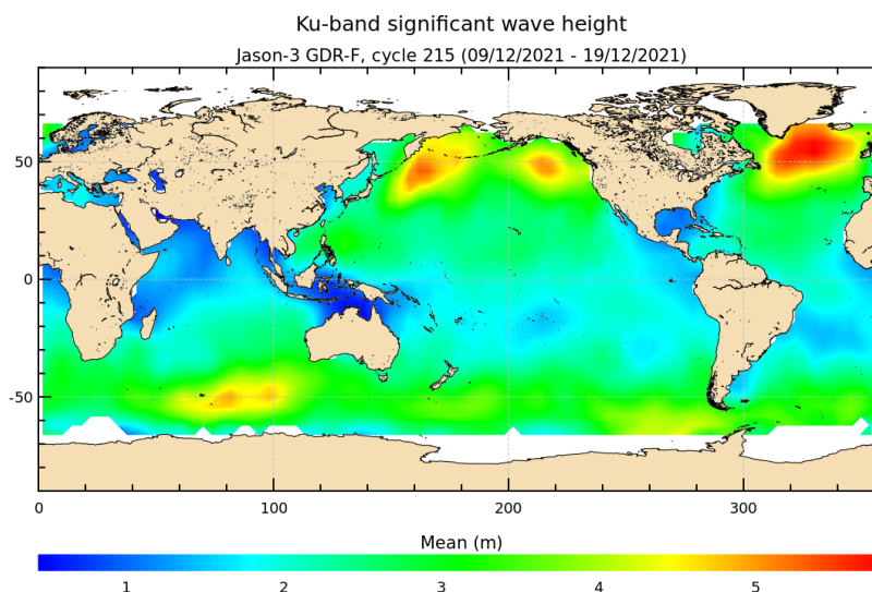
FIGURE 5 – Significant wave height for cycle 215.
