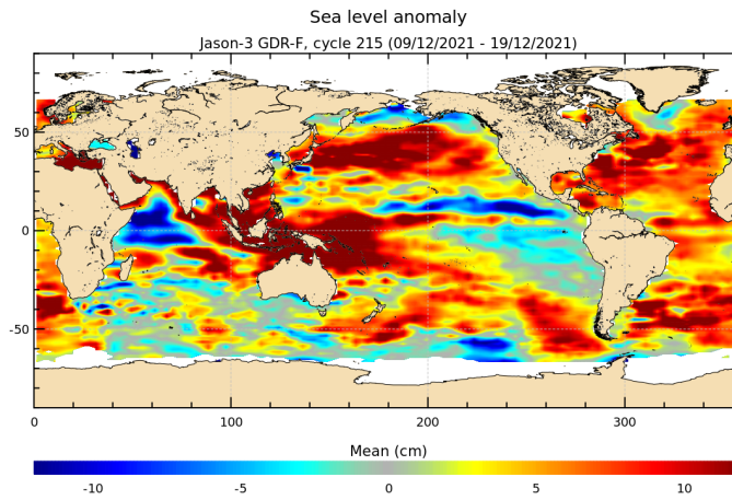
FIGURE 18 – Sea level anomaly relative to MSS for cycle 215.
