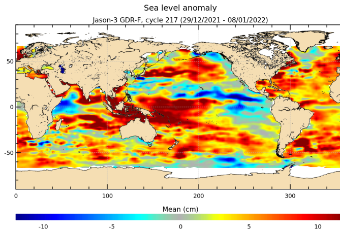
FIGURE 18 – Sea level anomaly relative to MSS for cycle 217.
