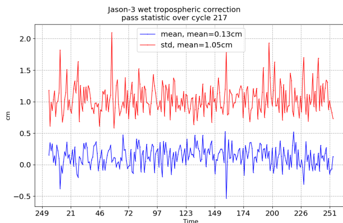
FIGURE 11 – Pass monitoring of wet troposphere differences between radiometer and ECMWF model for Jason-3 cycle 217
