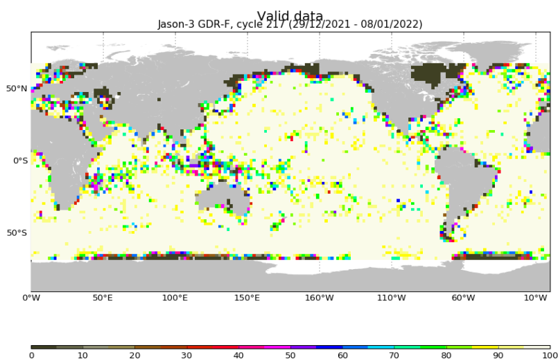
FIGURE 3 – Percentage of valid measurements for cycle 217.
