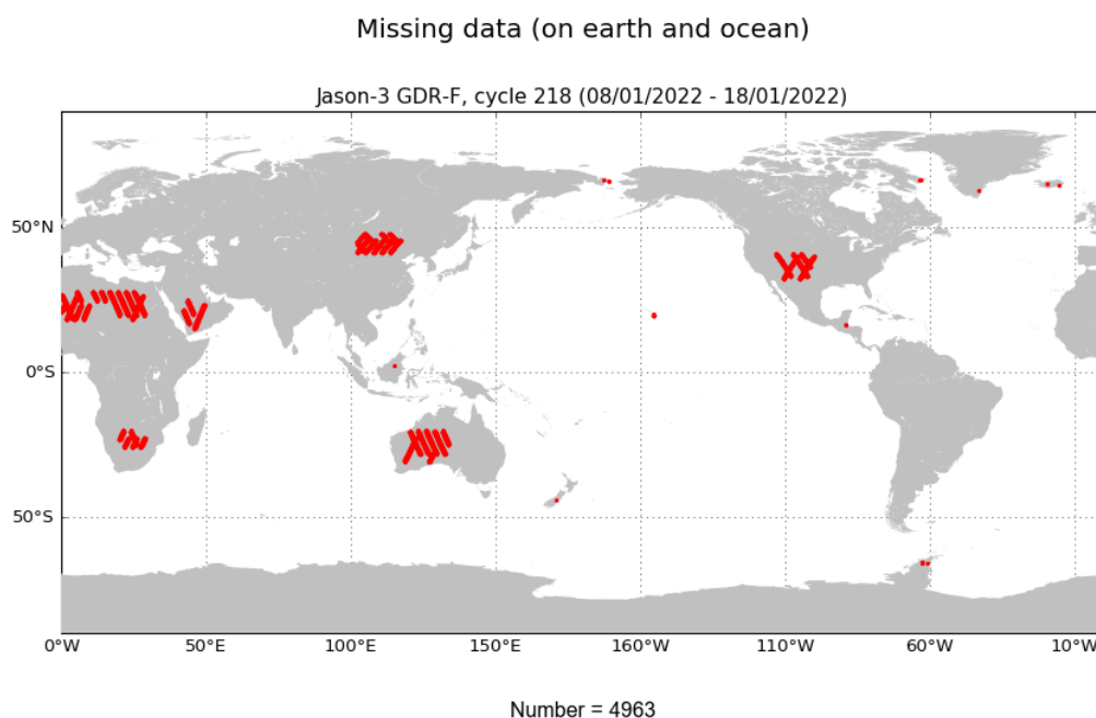
FIGURE 1 – Missing measurements for cycle 218.
