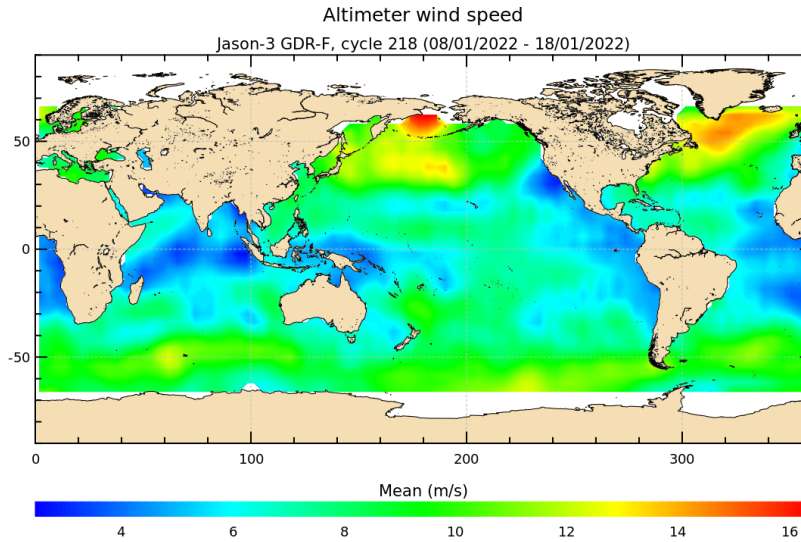
FIGURE 9 – Altimeter wind speed for cycle 218.
