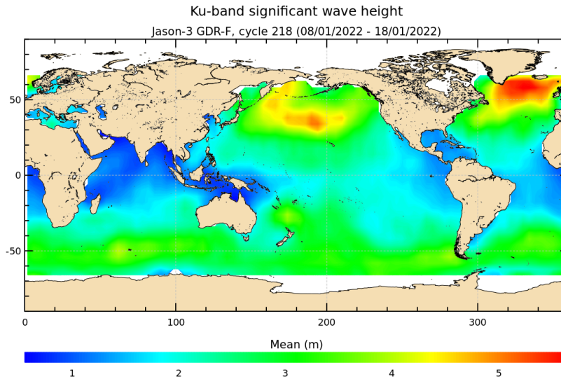
FIGURE 5 – Significant wave height for cycle 218.
