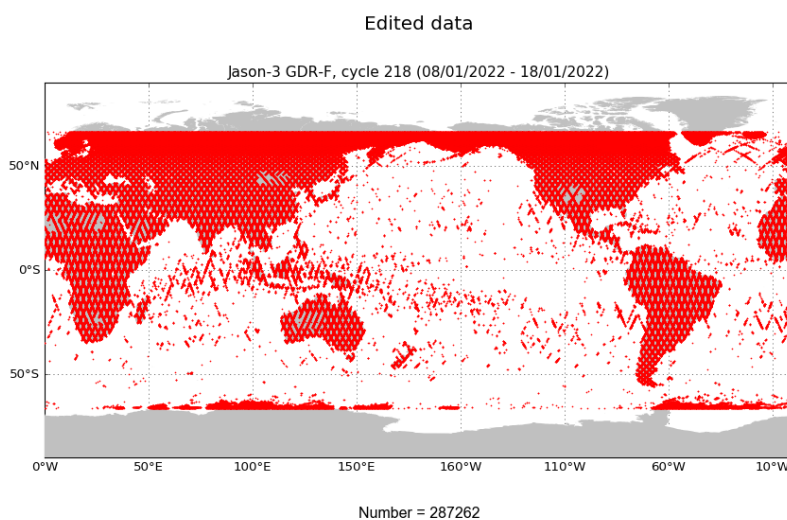
FIGURE 2 – Edited measurements for cycle 218.
