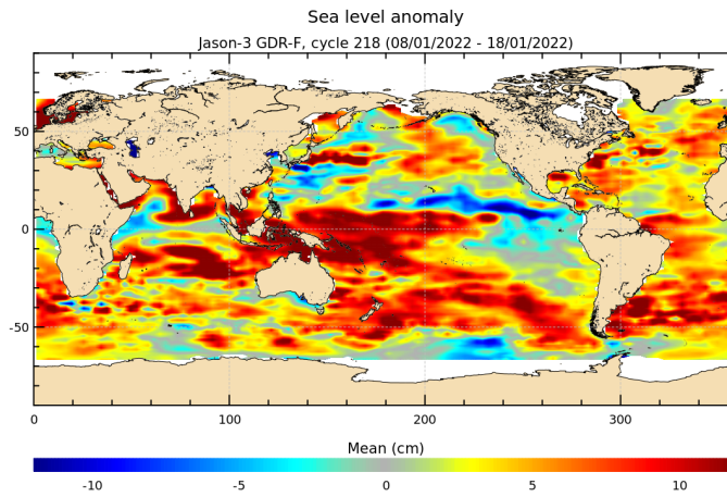
FIGURE 18 – Sea level anomaly relative to MSS for cycle 218.
