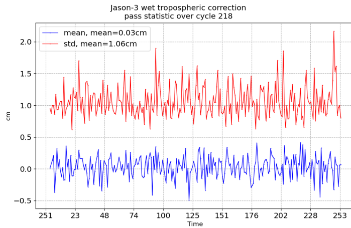
FIGURE 11 – Pass monitoring of wet troposphere differences between radiometer and ECMWF model for Jason-3 cycle 218
