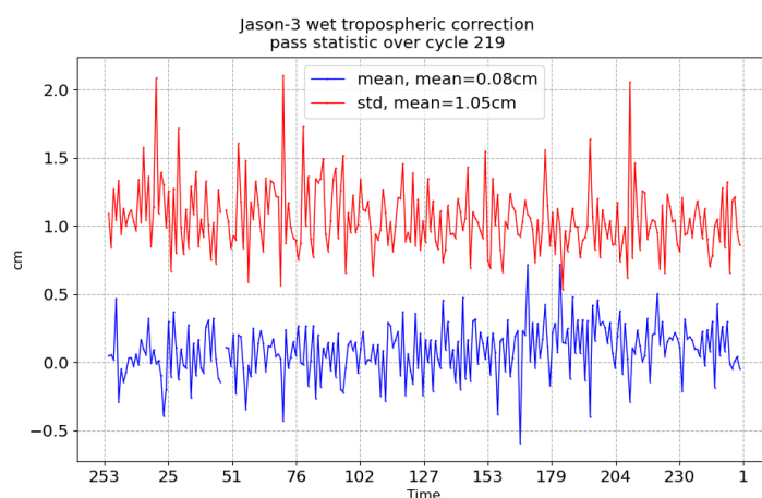
FIGURE 11 – Pass monitoring of wet troposphere differences between radiometer and ECMWF model for Jason-3 cycle 219
