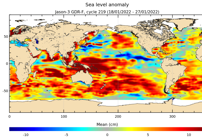
FIGURE 18 – Sea level anomaly relative to MSS for cycle 219.
