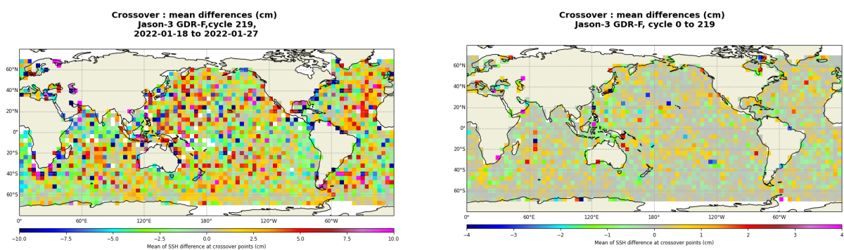
FIGURE 13 – Mean SSH at crossovers for cycle 219 (left) and over the whole Jason-3 period (right).
