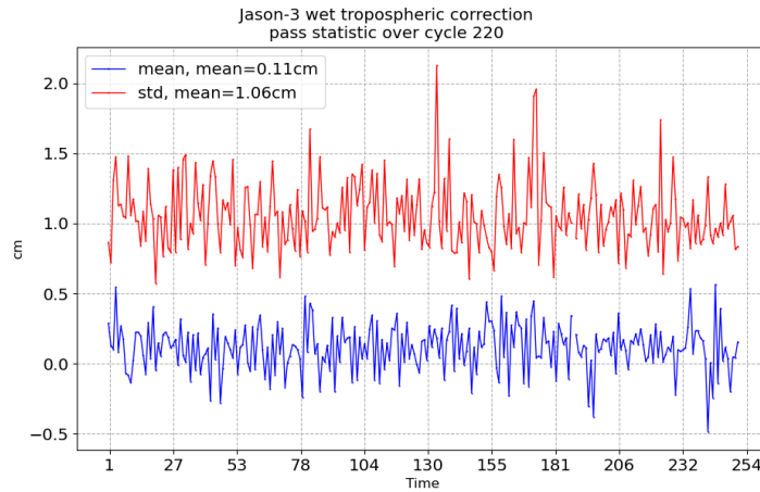
FIGURE 11 – Pass monitoring of wet troposphere differences between radiometer and ECMWF model for Jason-3 cycle 220
