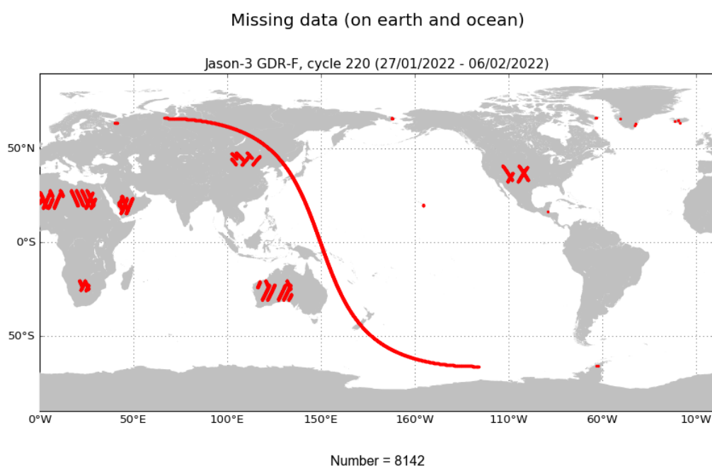
FIGURE 1 – Missing measurements for cycle 220.
