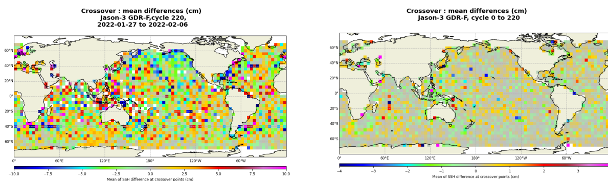
FIGURE 13 – Mean SSH at crossovers for cycle 220 (left) and over the whole Jason-3 period (right).
