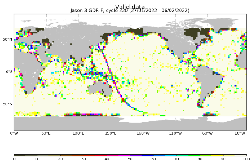
FIGURE 3 – Percentage of valid measurements for cycle 220.
