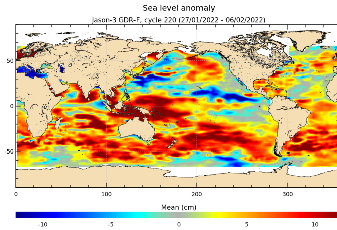
FIGURE 18 – Sea level anomaly relative to MSS for cycle 220.
