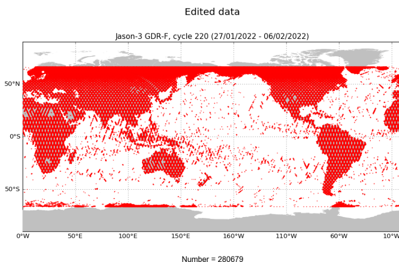
FIGURE 2 – Edited measurements for cycle 220.
