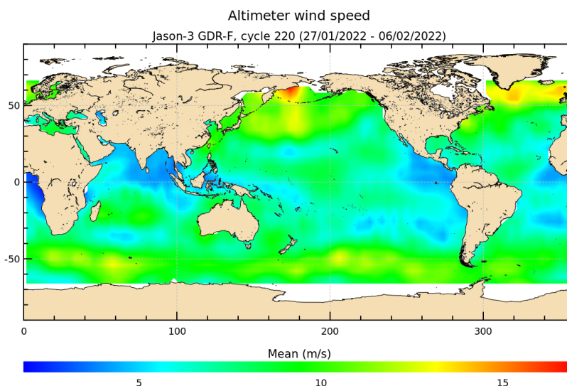
FIGURE 9 – Altimeter wind speed for cycle 220.
