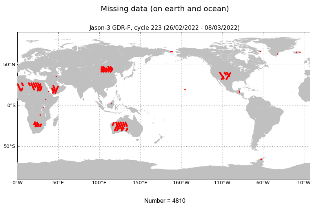
FIGURE 1 – Missing measurements for cycle 223.
