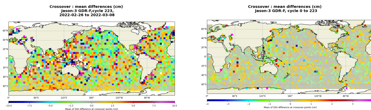
FIGURE 13 – Mean SSH at crossovers for cycle 223 (left) and over the whole Jason-3 period (right).
