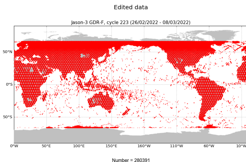
FIGURE 2 – Edited measurements for cycle 223.
