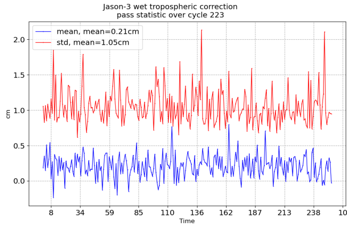
FIGURE 11 – Pass monitoring of wet troposphere differences between radiometer and ECMWF model for Jason-3 cycle 223
