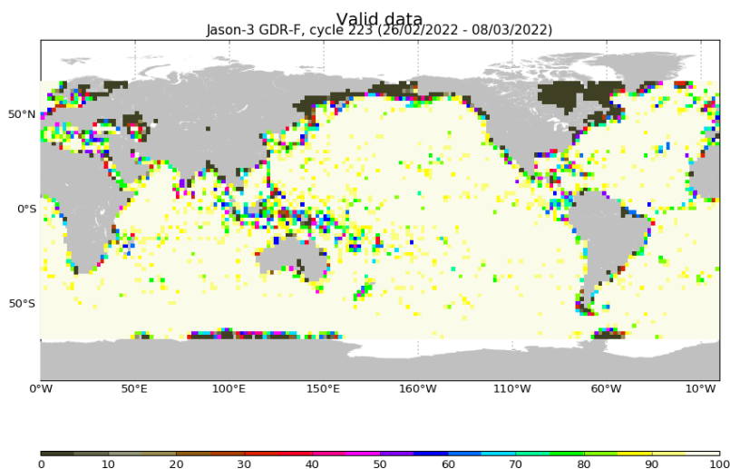
FIGURE 3 – Percentage of valid measurements for cycle 223.
