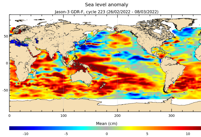
FIGURE 18 – Sea level anomaly relative to MSS for cycle 223.
