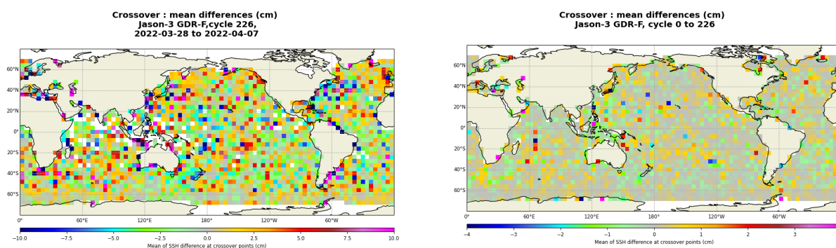
FIGURE 13 – Mean SSH at crossovers for cycle 226 (left) and over the whole Jason-3 period (right).
