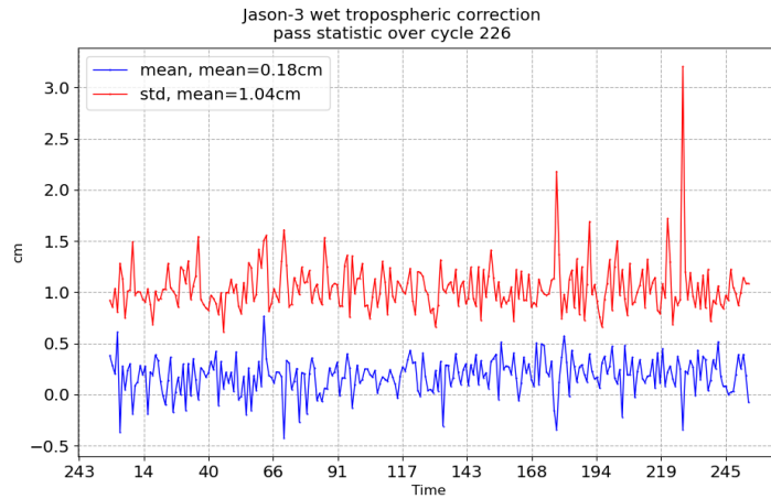
FIGURE 11 – Pass monitoring of wet troposphere differences between radiometer and ECMWF model for Jason-3 cycle 226
