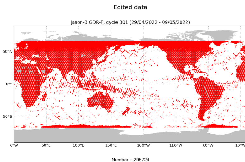
FIGURE 2 – Edited measurements for cycle 301.
