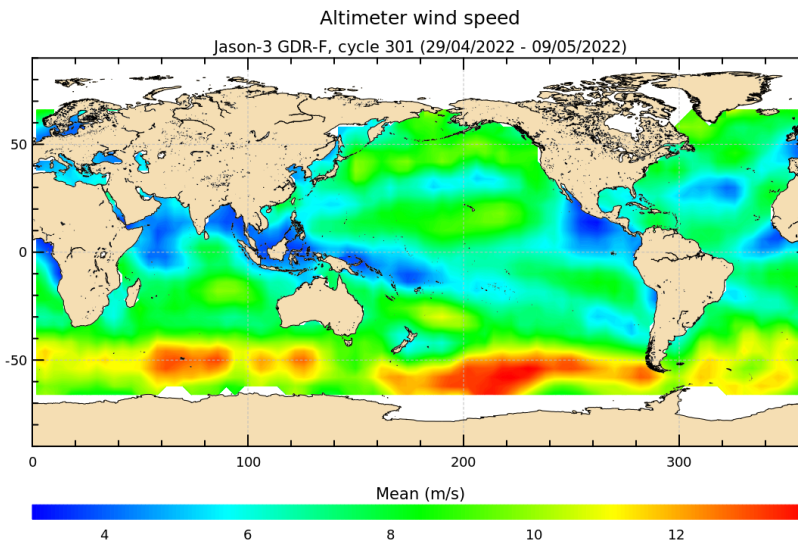
FIGURE 9 – Altimeter wind speed for cycle 301.
