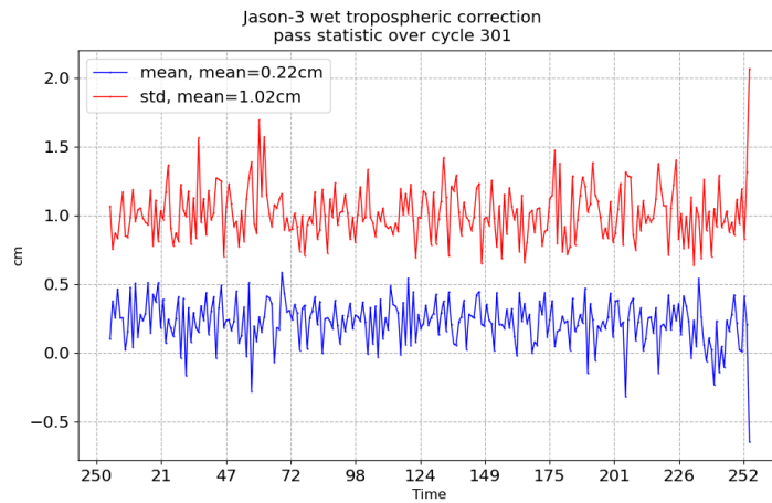
FIGURE 11 – Pass monitoring of wet troposphere differences between radiometer and ECMWF model for Jason-3 cycle 301
