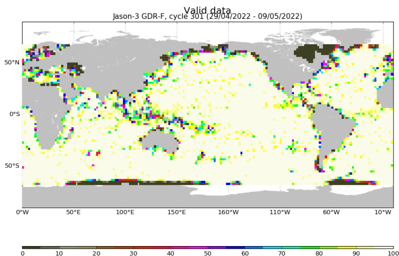
FIGURE 3 – Percentage of valid measurements for cycle 301.
