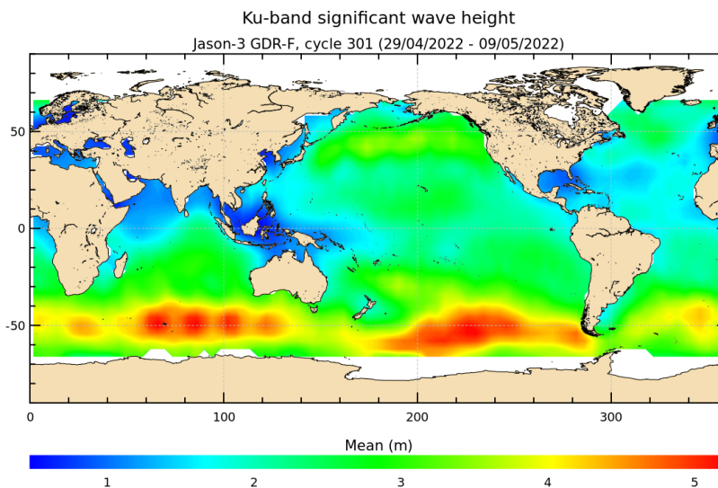
FIGURE 5 – Significant wave height for cycle 301.
