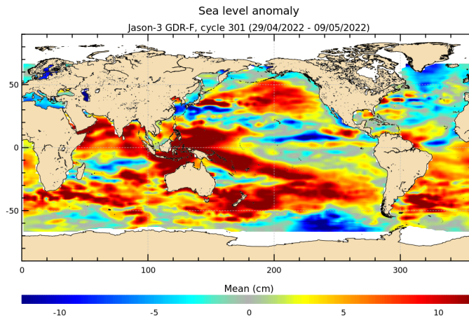
FIGURE 18 – Sea level anomaly relative to MSS for cycle 301.
