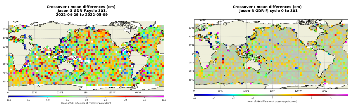
FIGURE 13 – Mean SSH at crossovers for cycle 301 (left) and over the whole Jason-3 period (right).
