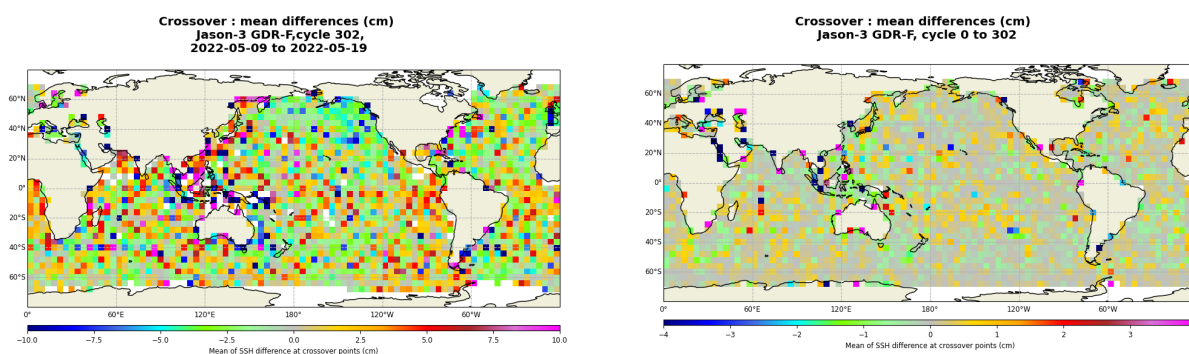
FIGURE 13 – Mean SSH at crossovers for cycle 302 (left) and over the whole Jason-3 period (right).
