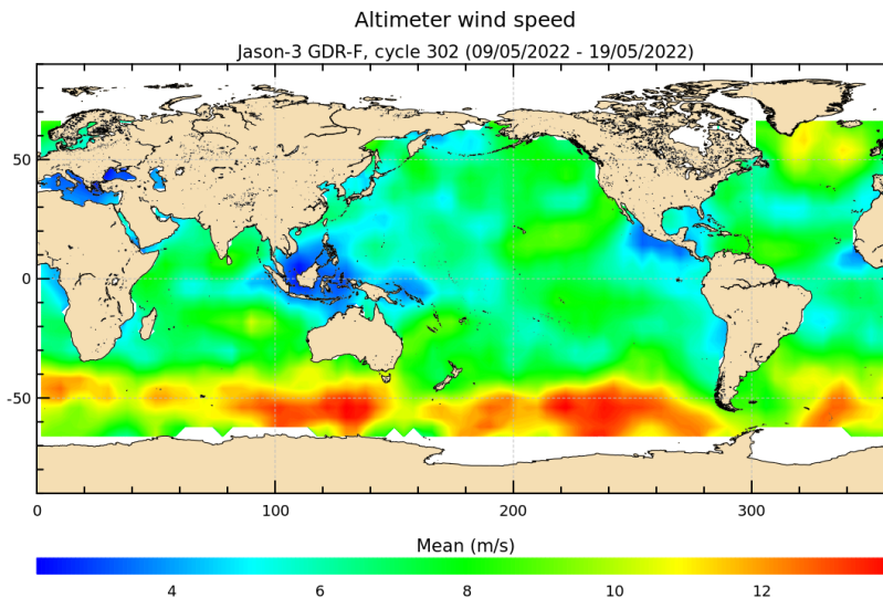
FIGURE 9 – Altimeter wind speed for cycle 302.
