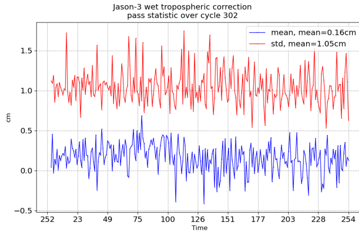
FIGURE 11 – Pass monitoring of wet troposphere differences between radiometer and ECMWF model for Jason-3 cycle 302
