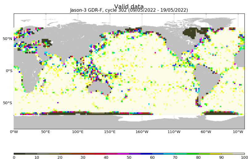
FIGURE 3 – Percentage of valid measurements for cycle 302.
