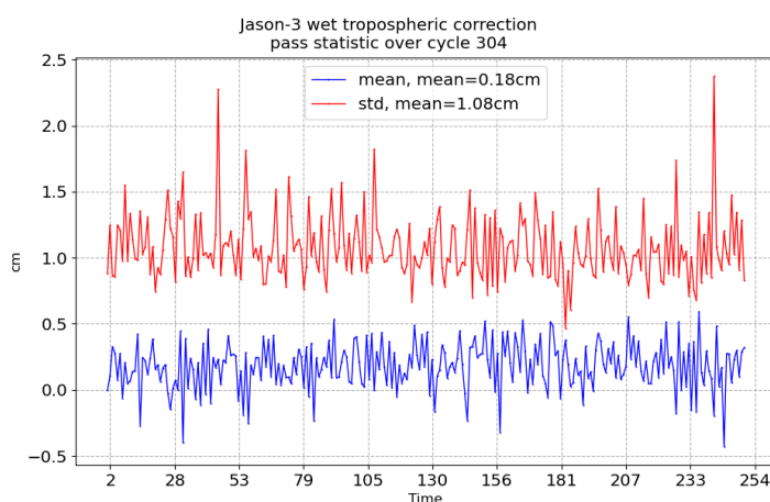
FIGURE 11 – Pass monitoring of wet troposphere differences between radiometer and ECMWF model for Jason-3 cycle 304
