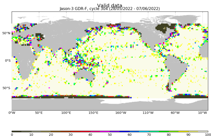
FIGURE 3 – Percentage of valid measurements for cycle 304.
