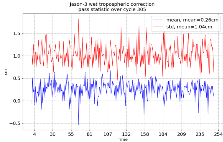
FIGURE 11 – Pass monitoring of wet troposphere differences between radiometer and ECMWF model for Jason-3 cycle 305
