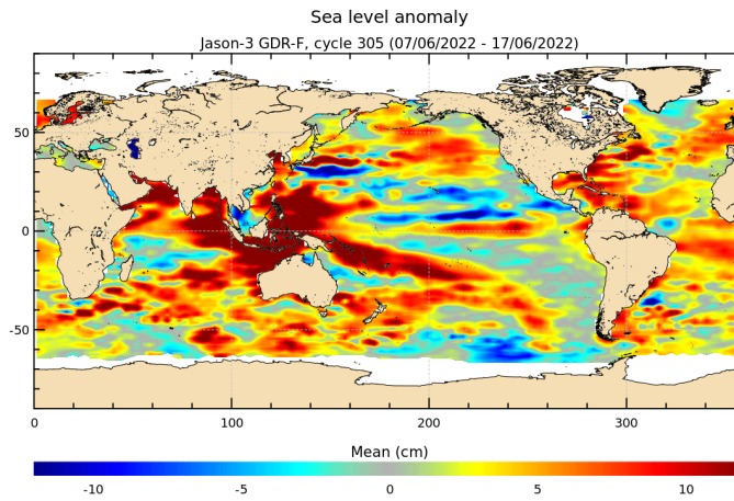
FIGURE 18 – Sea level anomaly relative to MSS for cycle 305.
