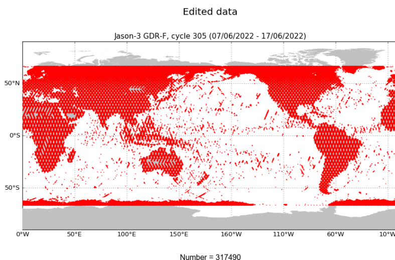
FIGURE 2 – Edited measurements for cycle 305.
