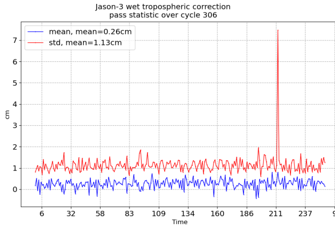
FIGURE 11 – Pass monitoring of wet troposphere differences between radiometer and ECMWF model for Jason-3 cycle 306
