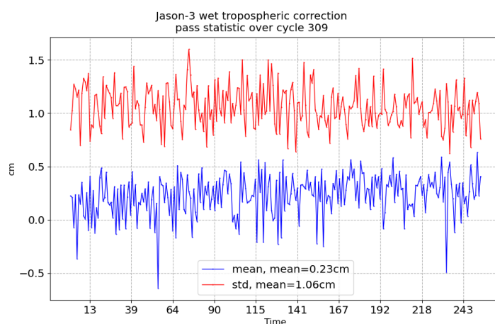
FIGURE 11 – Pass monitoring of wet troposphere differences between radiometer and ECMWF model for Jason-3 cycle 309
