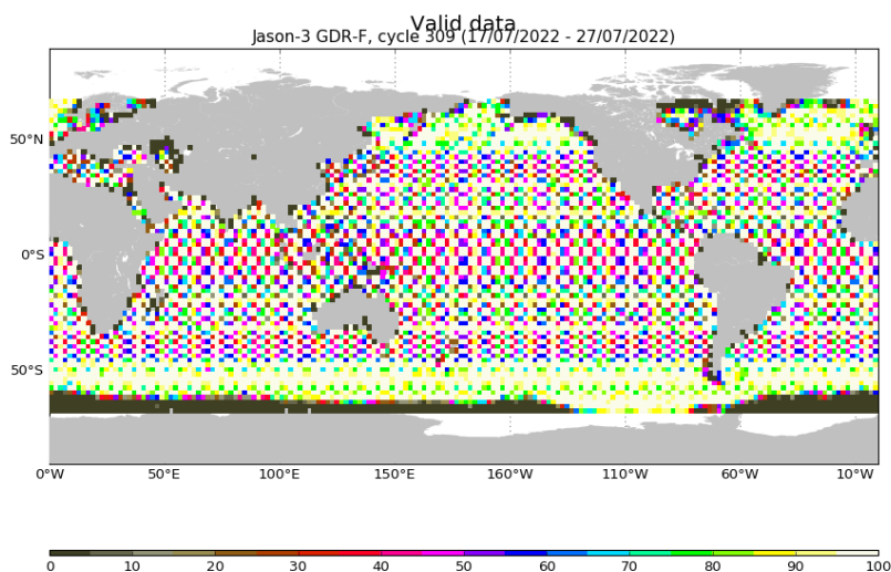
FIGURE 3 – Percentage of valid measurements for cycle 309.
