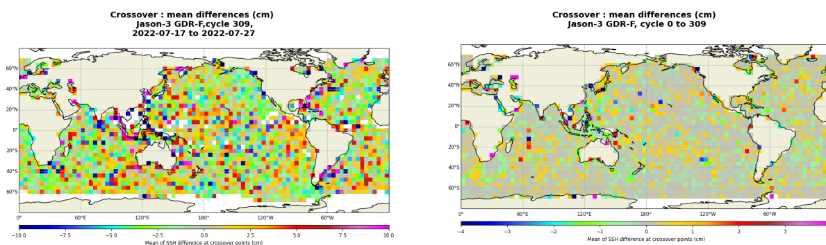
FIGURE 13 – Mean SSH at crossovers for cycle 309 (left) and over the whole Jason-3 period (right).
