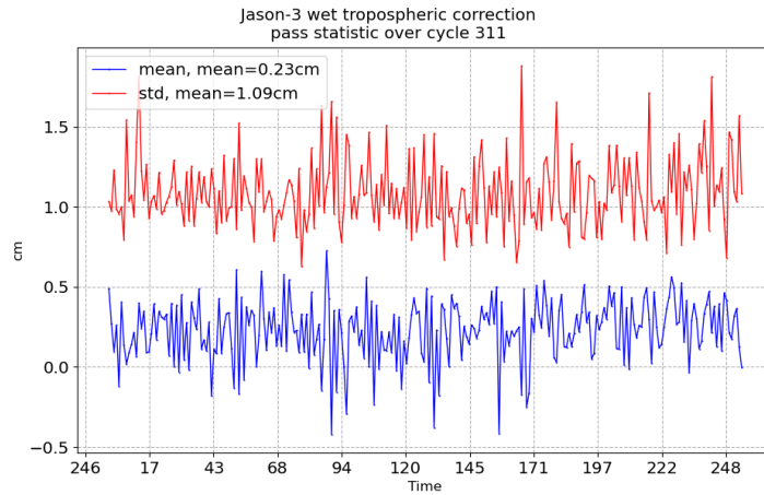
FIGURE 11 – Pass monitoring of wet troposphere differences between radiometer and ECMWF model for Jason-3 cycle 311
