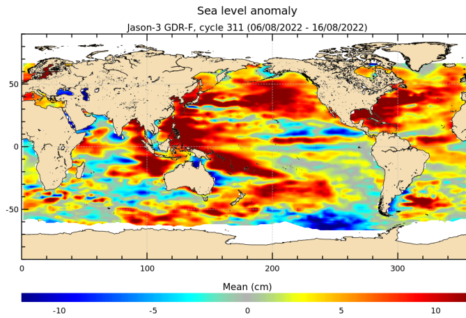
FIGURE 18 – Sea level anomaly relative to MSS for cycle 311.
