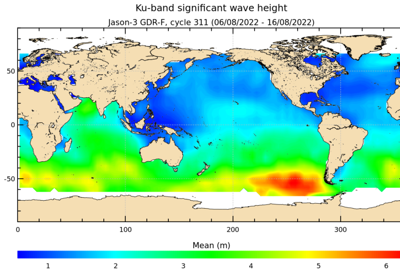
FIGURE 5 – Significant wave height for cycle 311.
