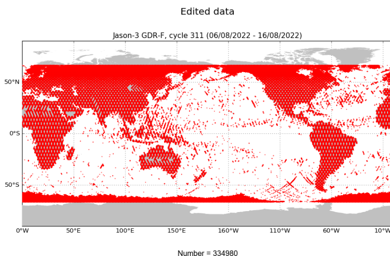
FIGURE 2 – Edited measurements for cycle 311.
