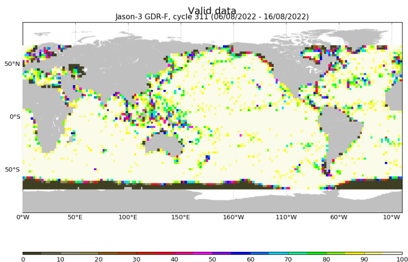
FIGURE 3 – Percentage of valid measurements for cycle 311.
