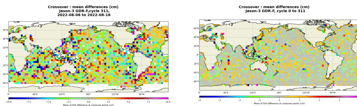
FIGURE 13 – Mean SSH at crossovers for cycle 311 (left) and over the whole Jason-3 period (right).
