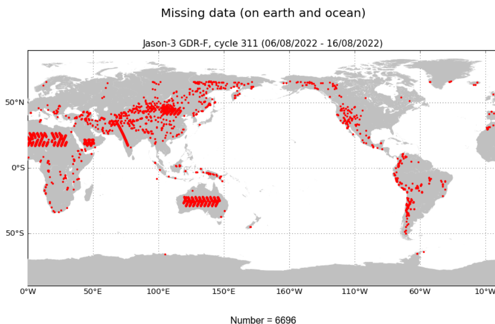
FIGURE 1 – Missing measurements for cycle 311.
