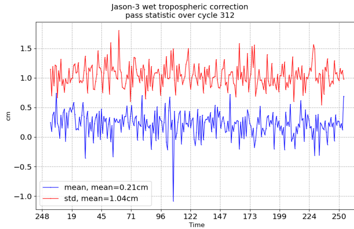
FIGURE 11 – Pass monitoring of wet troposphere differences between radiometer and ECMWF model for Jason-3 cycle 312
