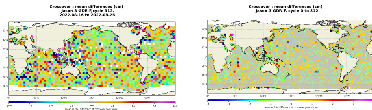
FIGURE 13 – Mean SSH at crossovers for cycle 312 (left) and over the whole Jason-3 period (right).
