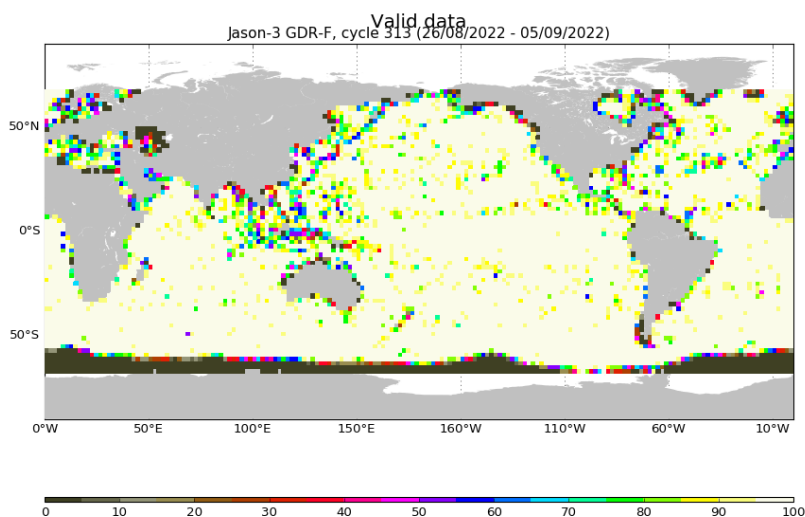
FIGURE 3 – Percentage of valid measurements for cycle 313.
