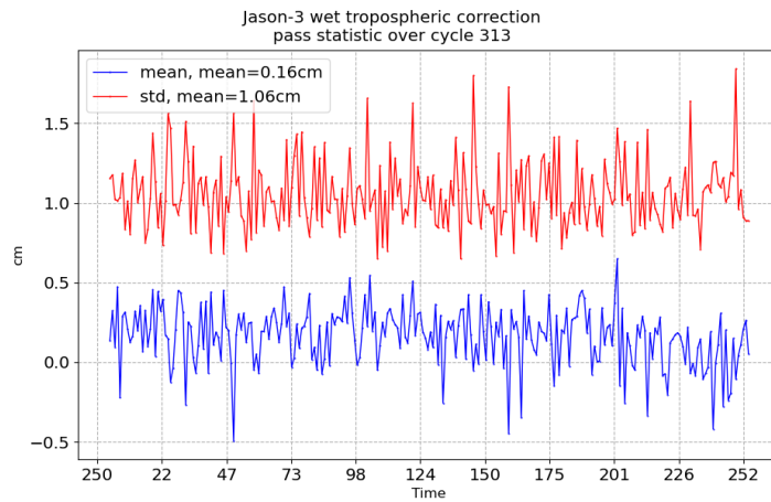
FIGURE 11 – Pass monitoring of wet troposphere differences between radiometer and ECMWF model for Jason-3 cycle 313
