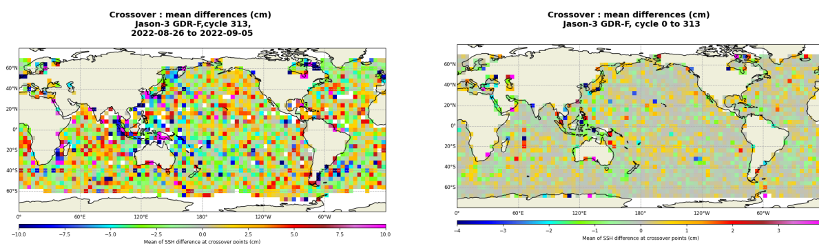
FIGURE 13 – Mean SSH at crossovers for cycle 313 (left) and over the whole Jason-3 period (right).
