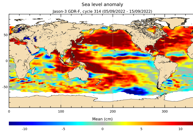
FIGURE 18 – Sea level anomaly relative to MSS for cycle 314.
