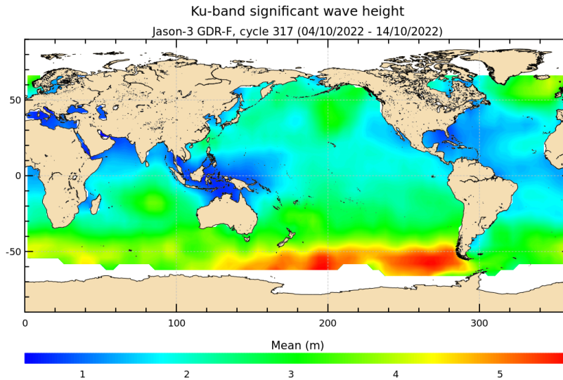
FIGURE 5 – Significant wave height for cycle 317.
