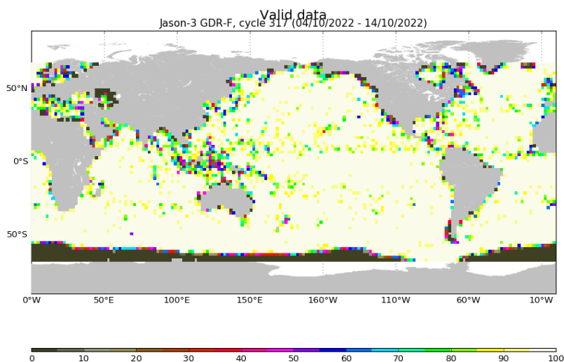
FIGURE 3 – Percentage of valid measurements for cycle 317.
