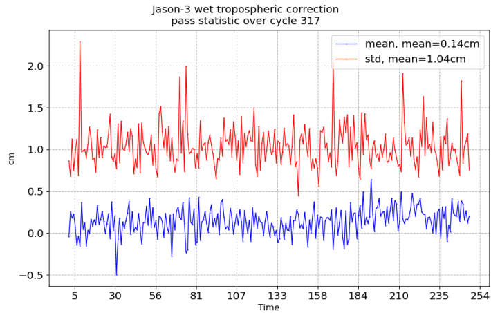
FIGURE 11 – Pass monitoring of wet troposphere differences between radiometer and ECMWF model for Jason-3 cycle 317
