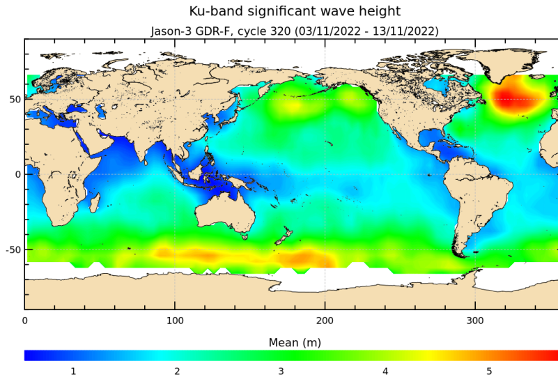
FIGURE 5 – Significant wave height for cycle 320.
