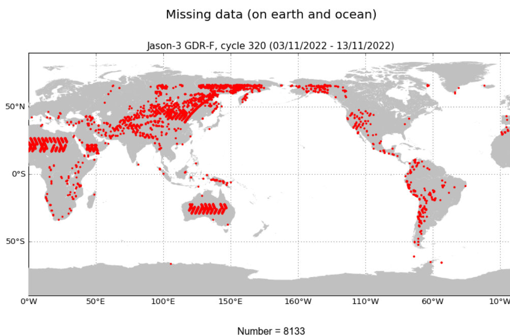
FIGURE 1 – Missing measurements for cycle 320.
