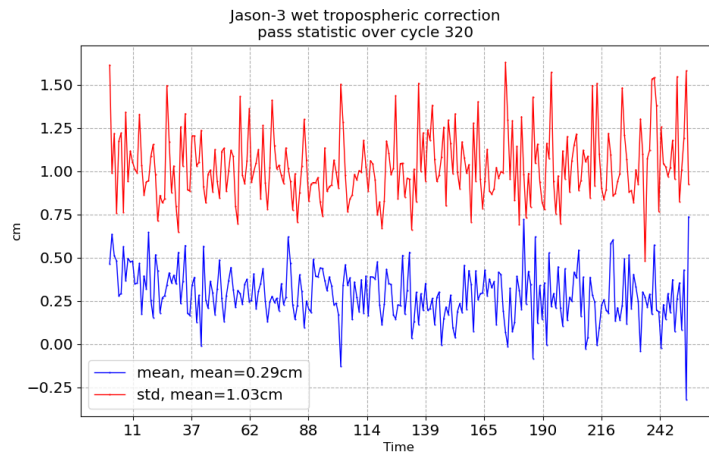
FIGURE 11 – Pass monitoring of wet troposphere differences between radiometer and ECMWF model for Jason-3 cycle 320
