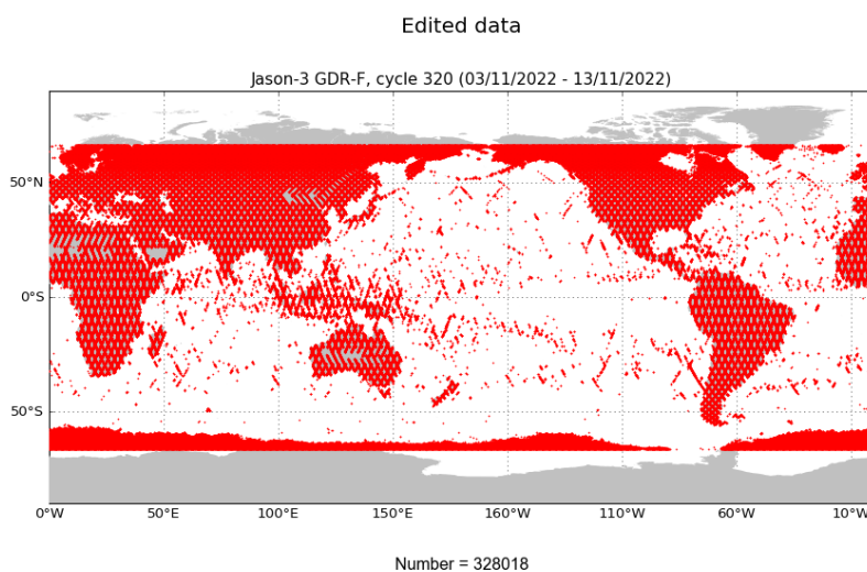
FIGURE 2 – Edited measurements for cycle 320.
