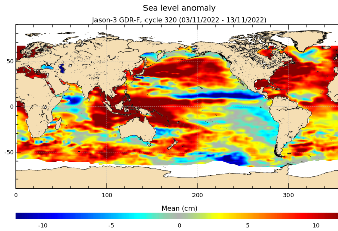
FIGURE 18 – Sea level anomaly relative to MSS for cycle 320.
