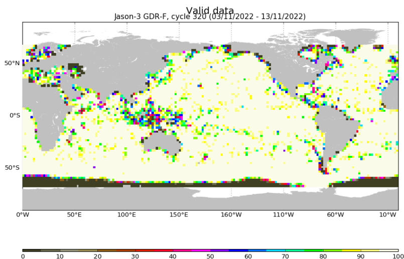
FIGURE 3 – Percentage of valid measurements for cycle 320.
