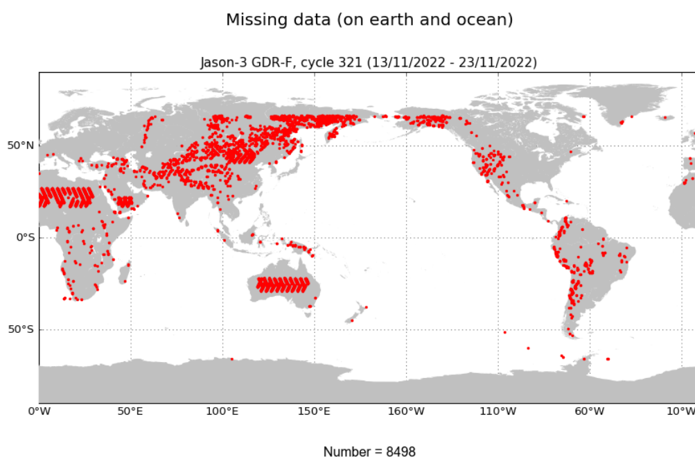
FIGURE 1 – Missing measurements for cycle 321.
