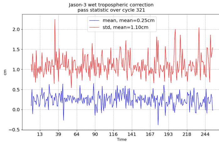
FIGURE 11 – Pass monitoring of wet troposphere differences between radiometer and ECMWF model for Jason-3 cycle 321
