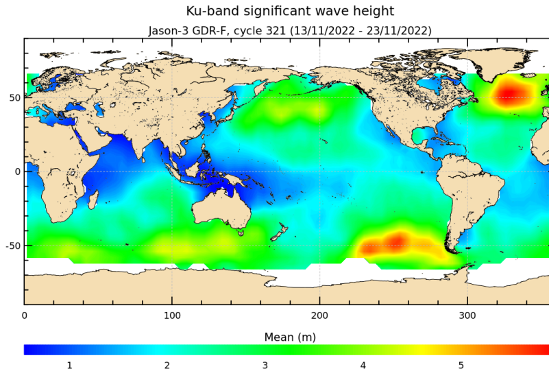
FIGURE 5 – Significant wave height for cycle 321.
