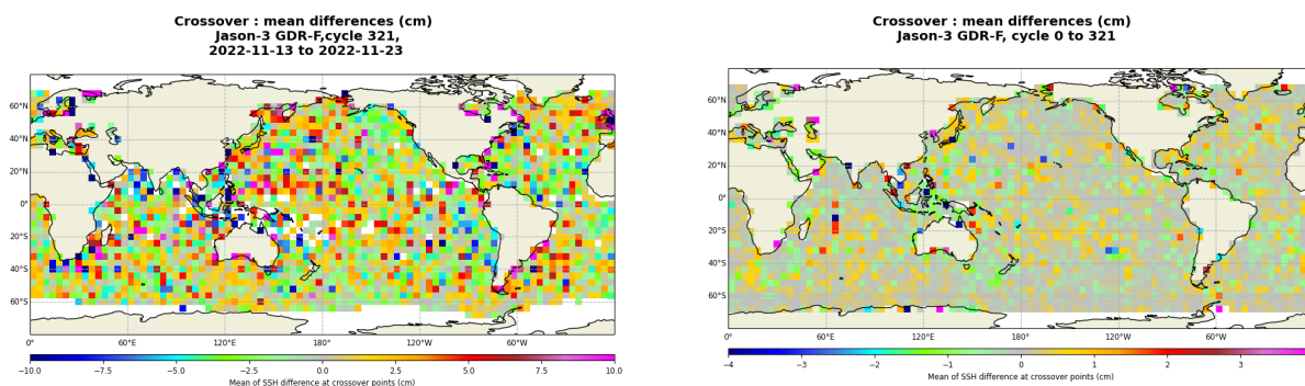
FIGURE 13 – Mean SSH at crossovers for cycle 321 (left) and over the whole Jason-3 period (right).
