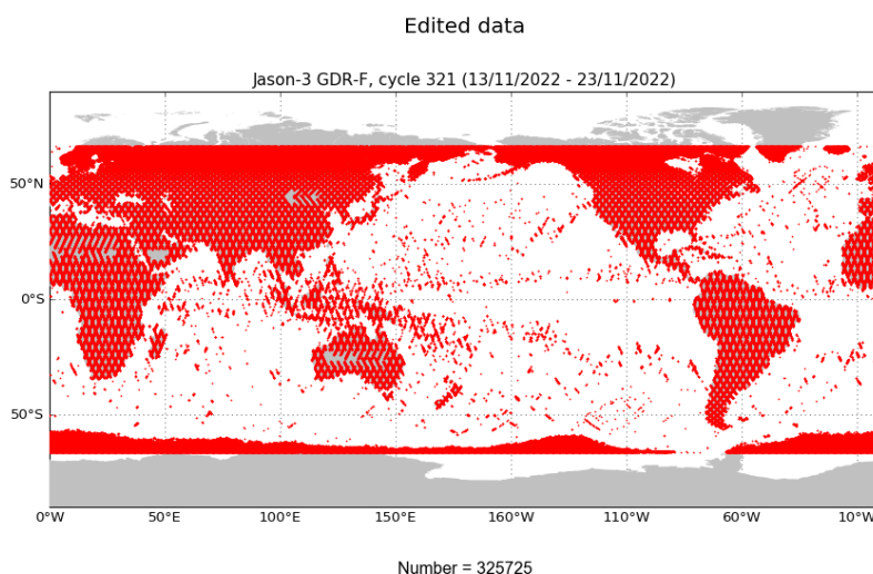
FIGURE 2 – Edited measurements for cycle 321.
