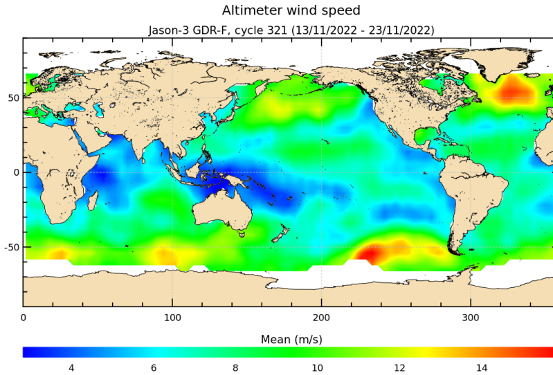
FIGURE 9 – Altimeter wind speed for cycle 321.
