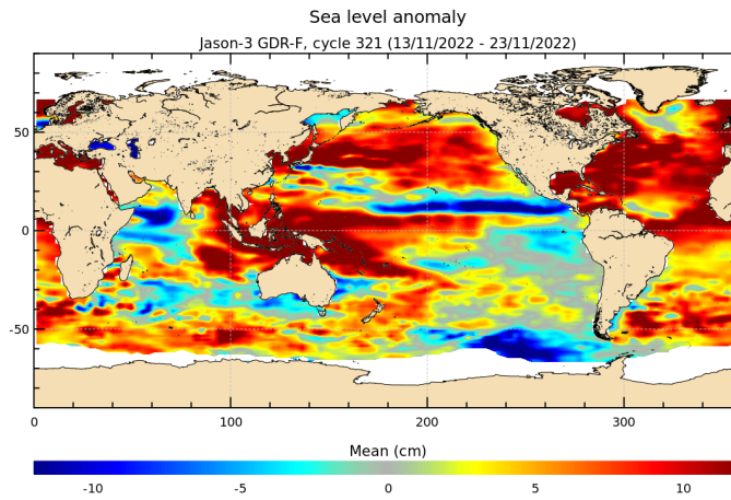
FIGURE 18 – Sea level anomaly relative to MSS for cycle 321.
