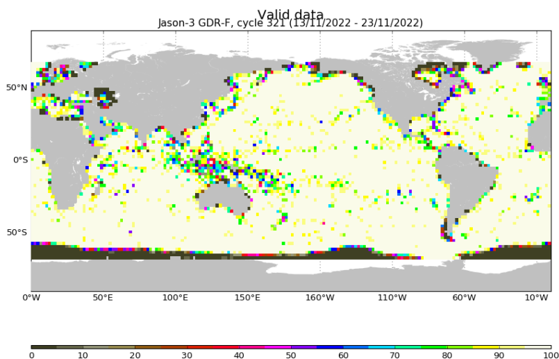
FIGURE 3 – Percentage of valid measurements for cycle 321.
