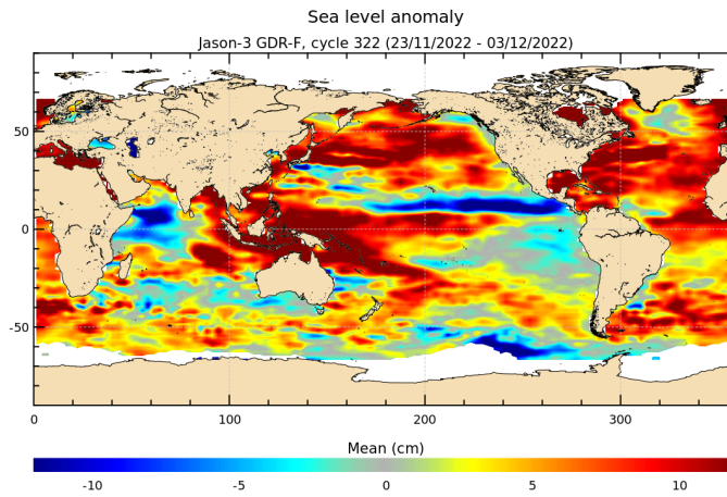
FIGURE 18 – Sea level anomaly relative to MSS for cycle 322.
