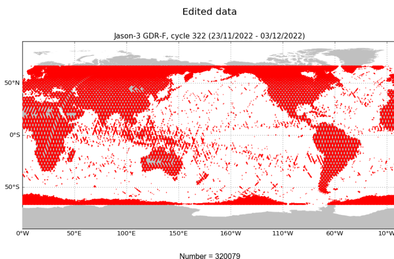
FIGURE 2 – Edited measurements for cycle 322.
