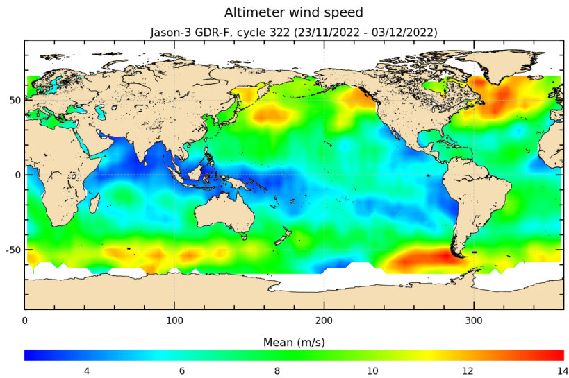
FIGURE 9 – Altimeter wind speed for cycle 322.
