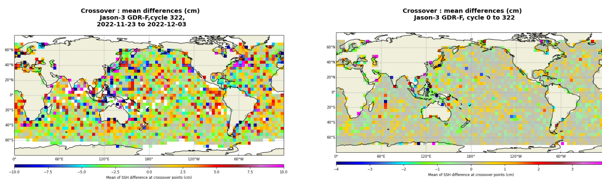
FIGURE 13 – Mean SSH at crossovers for cycle 322 (left) and over the whole Jason-3 period (right).
