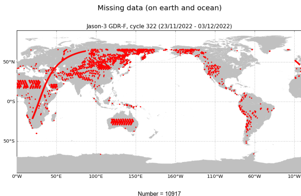
FIGURE 1 – Missing measurements for cycle 322.
