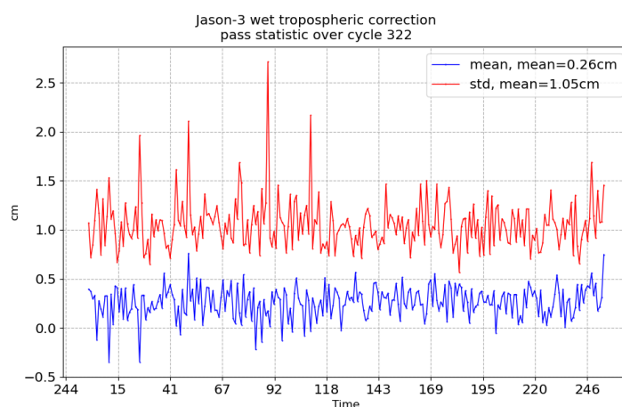
FIGURE 11 – Pass monitoring of wet troposphere differences between radiometer and ECMWF model for Jason-3 cycle 322
