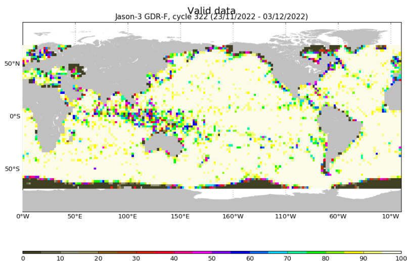
FIGURE 3 – Percentage of valid measurements for cycle 322.
